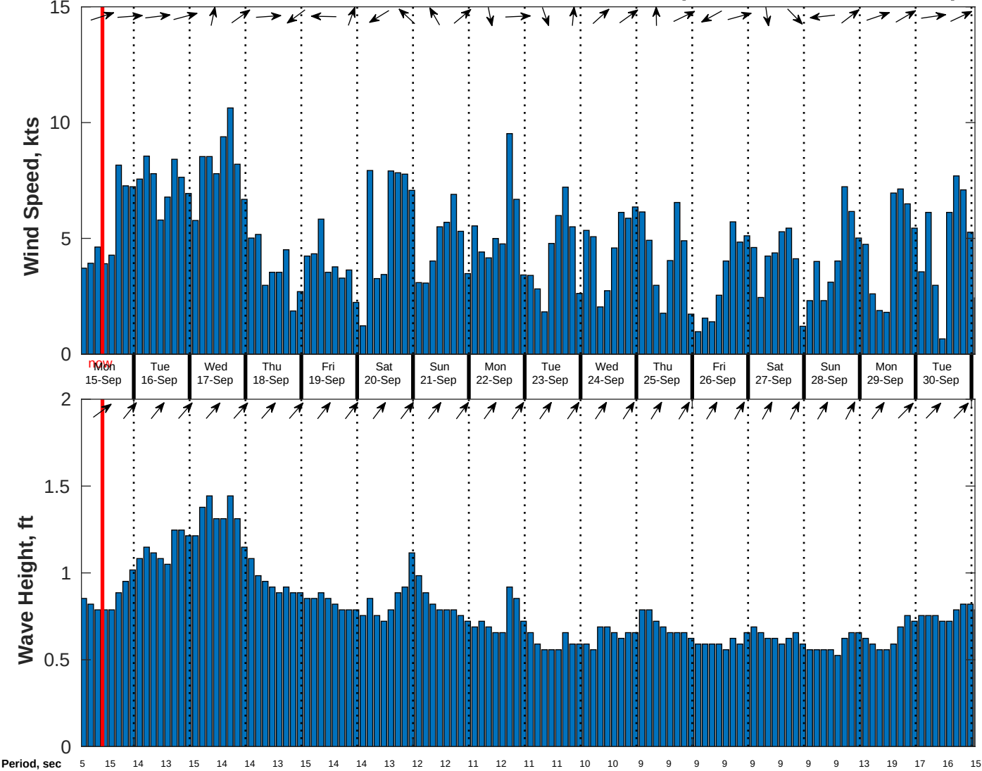
Wind & Wave Forecast for CSA (ONHYM) PPL EBS - Guinea from 14-Sep-2025 01:00:00 to 30-Sep-2025 01:00:00
