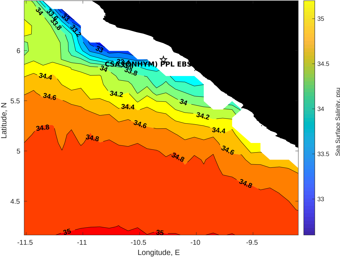
Surface Salinity for CSA (ONHYM) PPL EBS - Liberia at 13-Sep-2025 00:00:00
