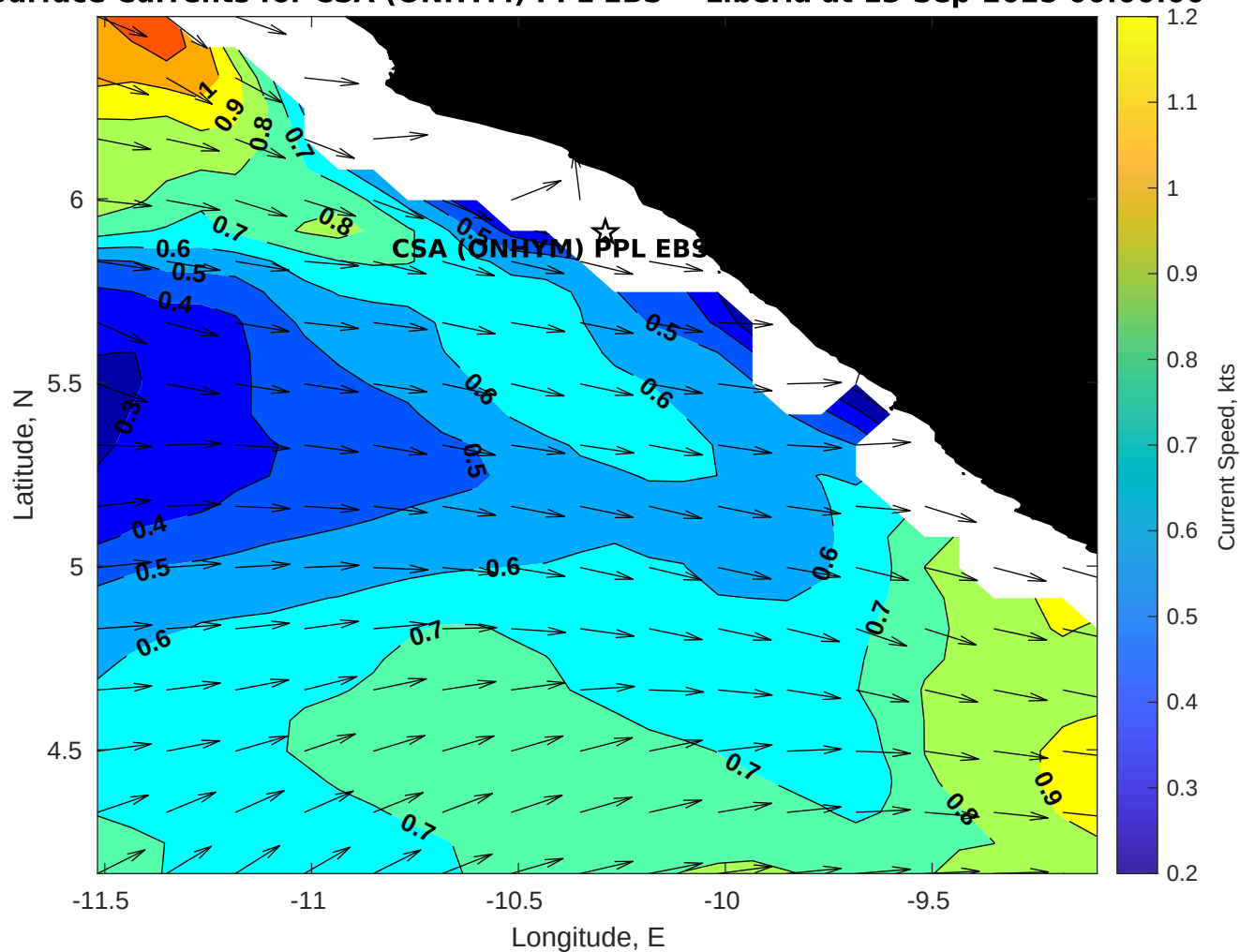
Surface Currents for CSA (ONHYM) PPL EBS - Liberia at 13-Sep-2025 00:00:00
