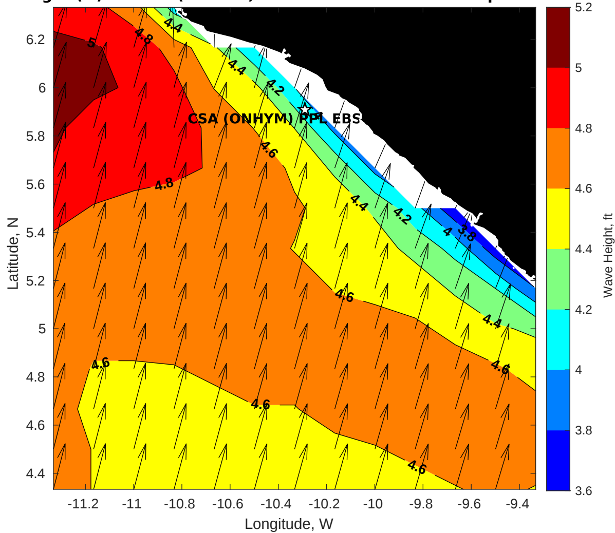
Wave Height (ft) for CSA (ONHYM) PPL EBS - Liberia at 14-Sep-2025 09:00:00
