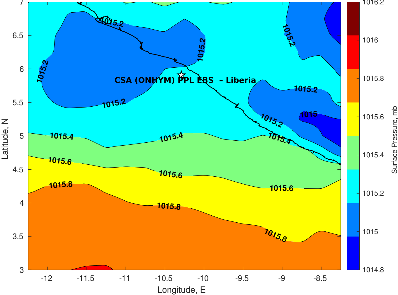
Surface Pressure (mb) for CSA (ONHYM) PPL EBS - Liberia at 14-Sep-2025 12:00:00
