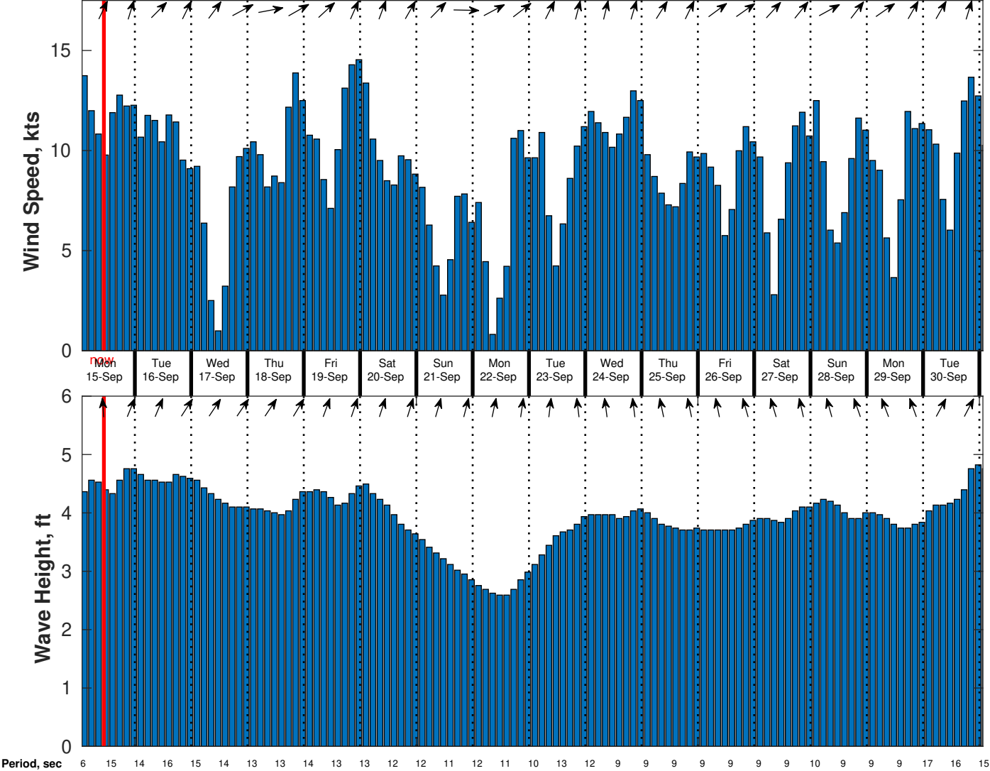
Wind & Wave Forecast for CSA (ONHYM) PPL EBS - Liberia from 14-Sep-2025 01:00:00 to 30-Sep-2025 01:00:00
