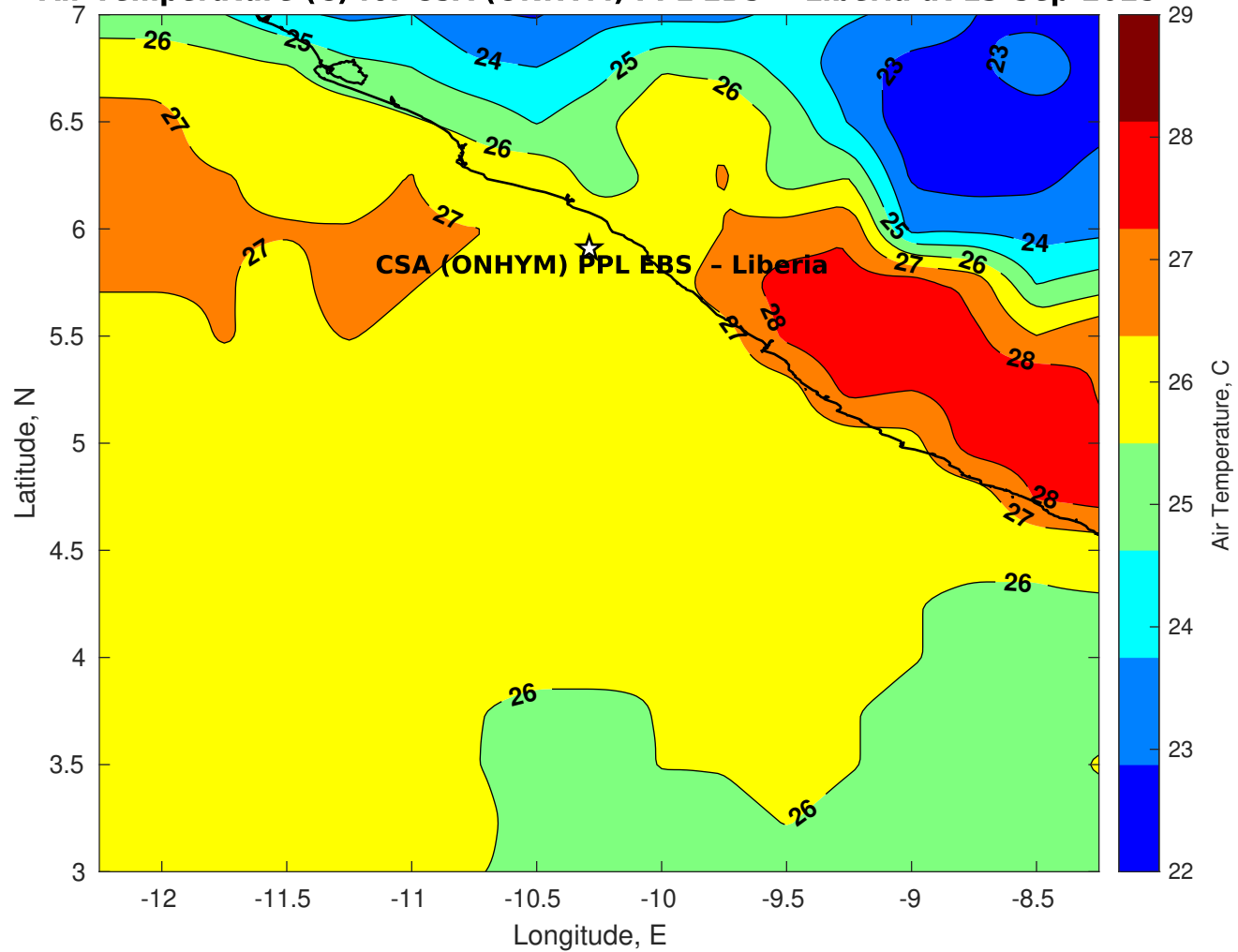
Air Temperature (C) for CSA (ONHYM) PPL EBS - Liberia at 13-Sep-2025
