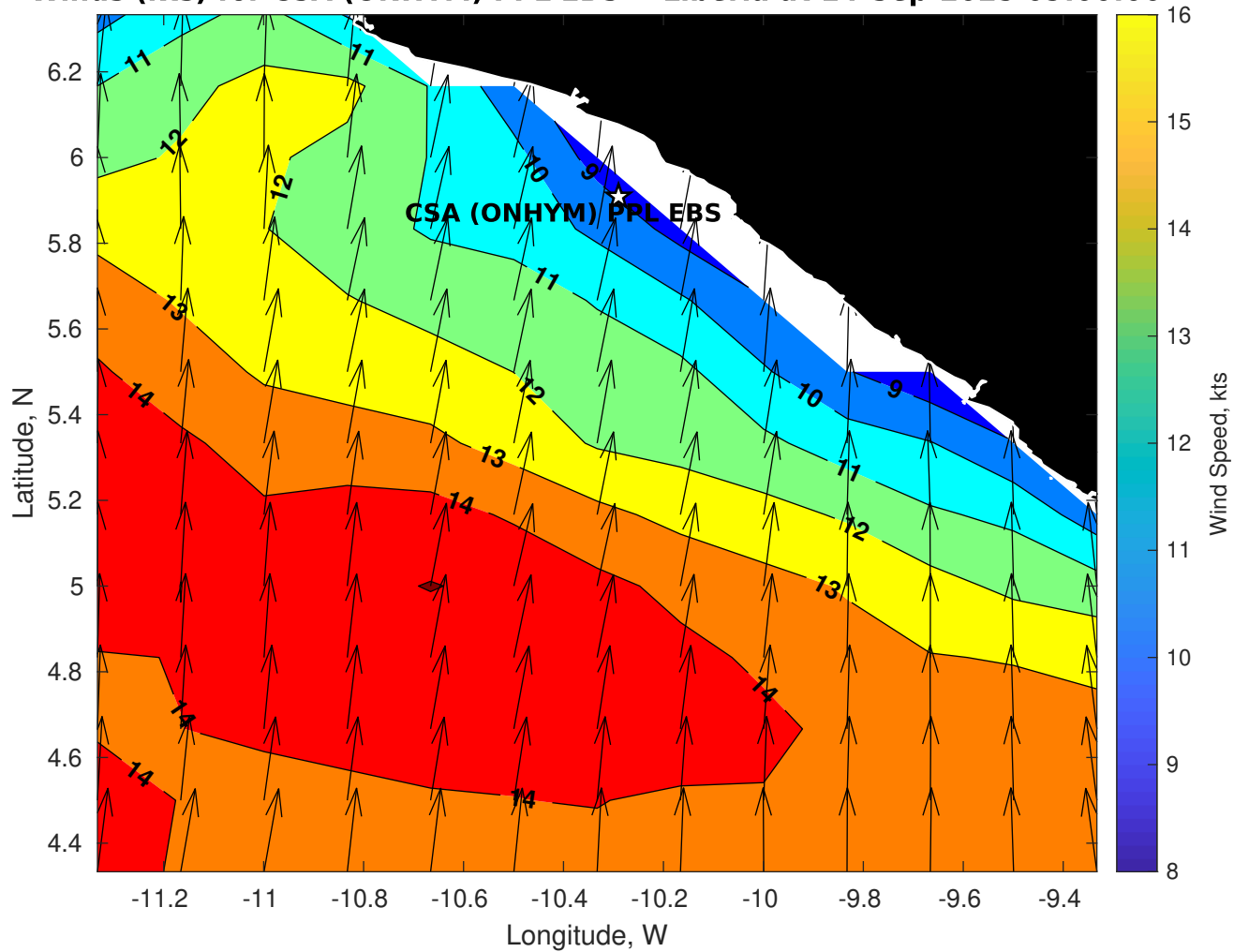
Winds (kts) for CSA (ONHYM) PPL EBS - Liberia at 14-Sep-2025 09:00:00
