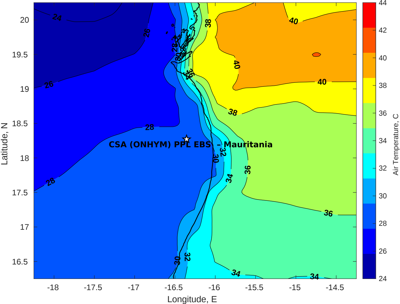
Air Temperature (C) for CSA (ONHYM) PPL EBS - Mauritania at 13-Sep-2025
