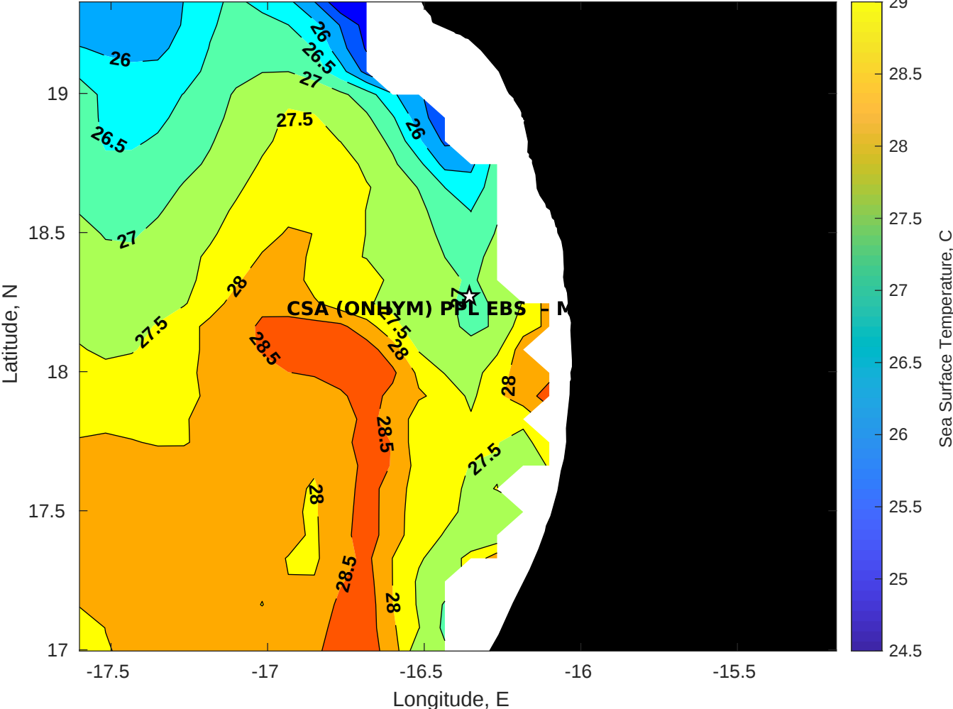
SST for CSA (ONHYM) PPL EBS - Mauritania at 13-Sep-2025 00:00:00
