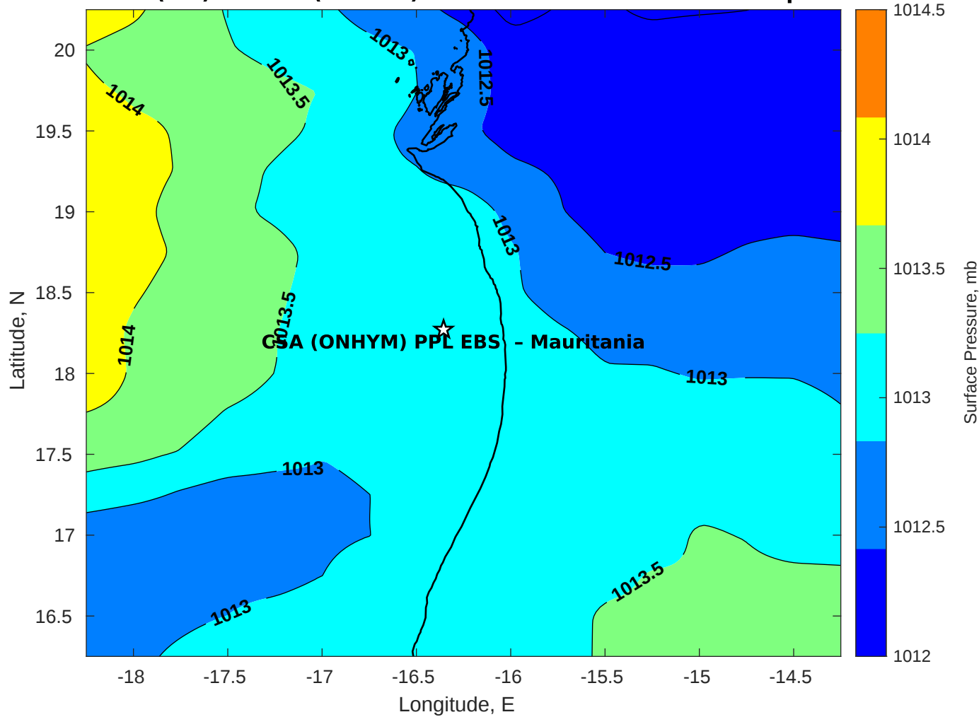
Surface Pressure (mb) for CSA (ONHYM) PPL EBS - Mauritania at 14-Sep-2025 12:00:00
