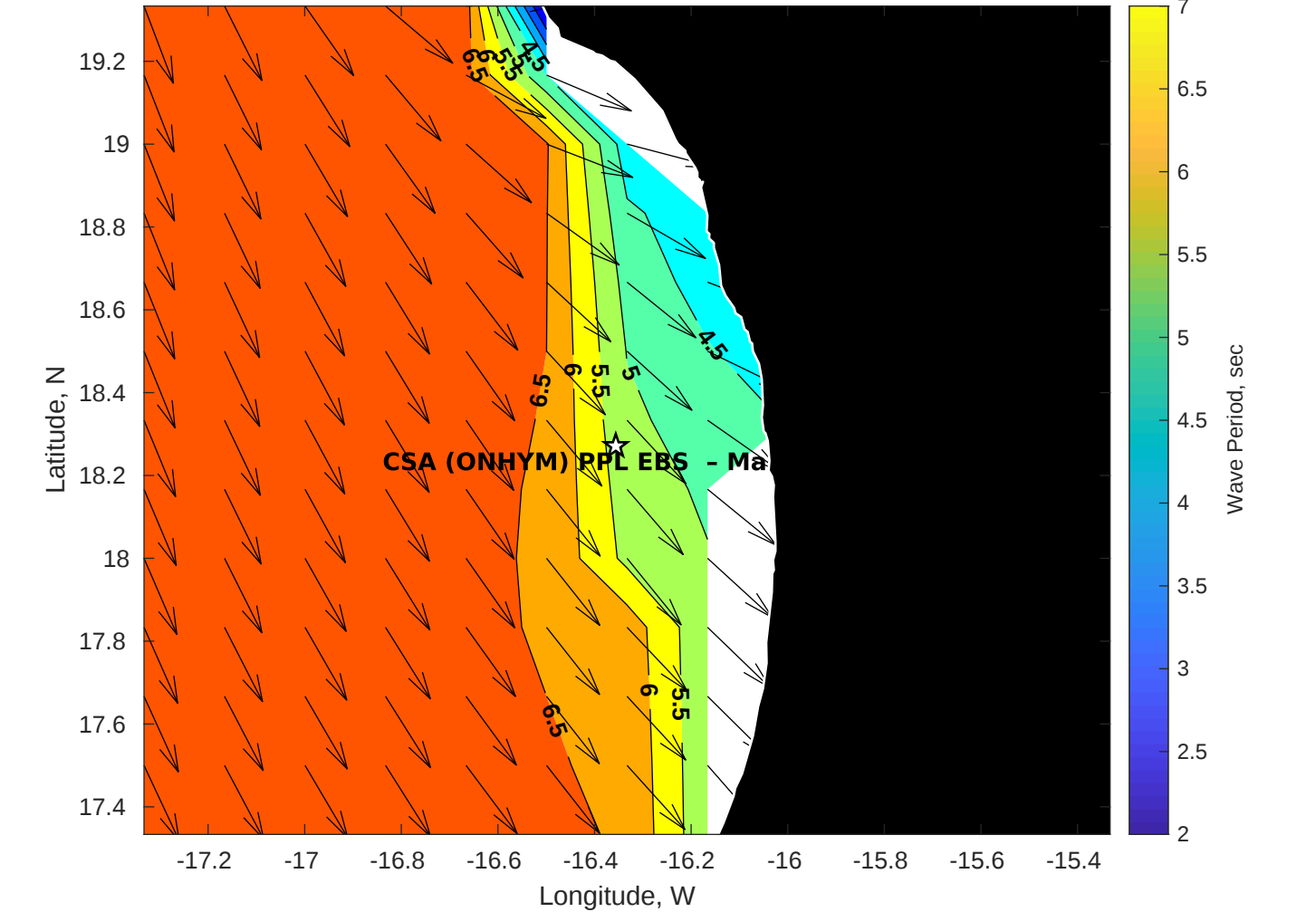
Wave Period (sec) for CSA (ONHYM) PPL EBS - Mauritania at 14-Sep-2025 09:00:00
