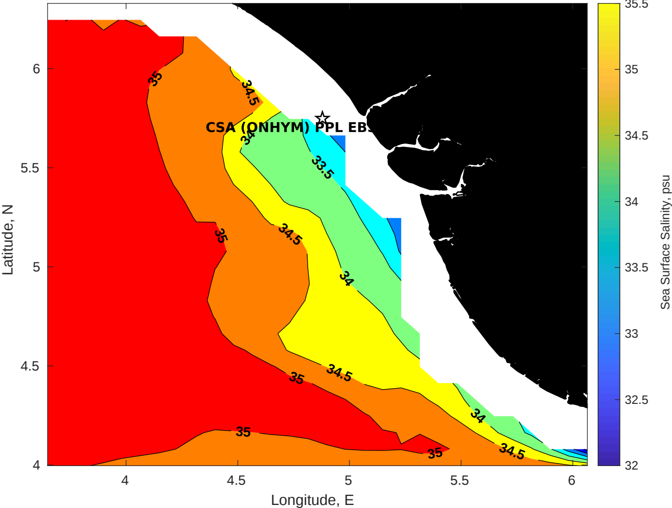
Surface Salinity for CSA (ONHYM) PPL EBS - Nigeria at 13-Sep-2025 00:00:00
