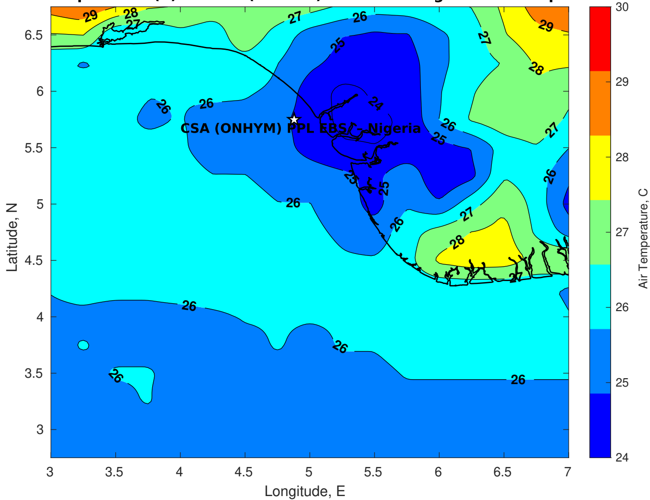
Air Temperature (C) for CSA (ONHYM) PPL EBS - Nigeria at 13-Sep-2025
