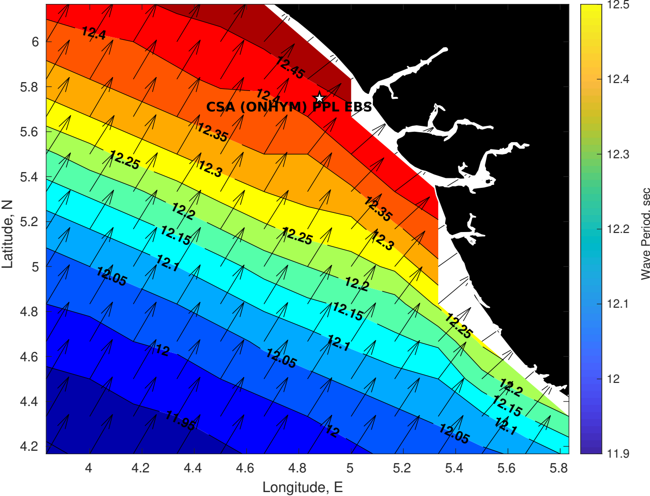
Wave Period (sec) for CSA (ONHYM) PPL EBS - Nigeria at 14-Sep-2025 09:00:00
