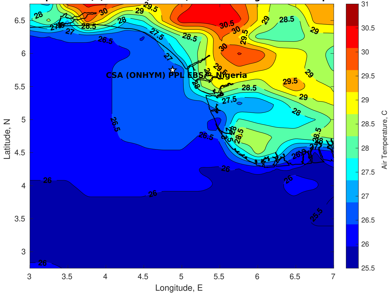
Air Temperature (C) for CSA (ONHYM) PPL EBS - Nigeria at 13-Sep-2025
