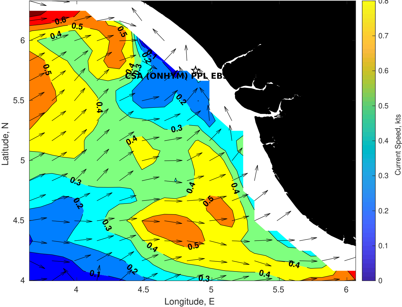
Surface Currents for CSA (ONHYM) PPL EBS - Nigeria at 13-Sep-2025 00:00:00
