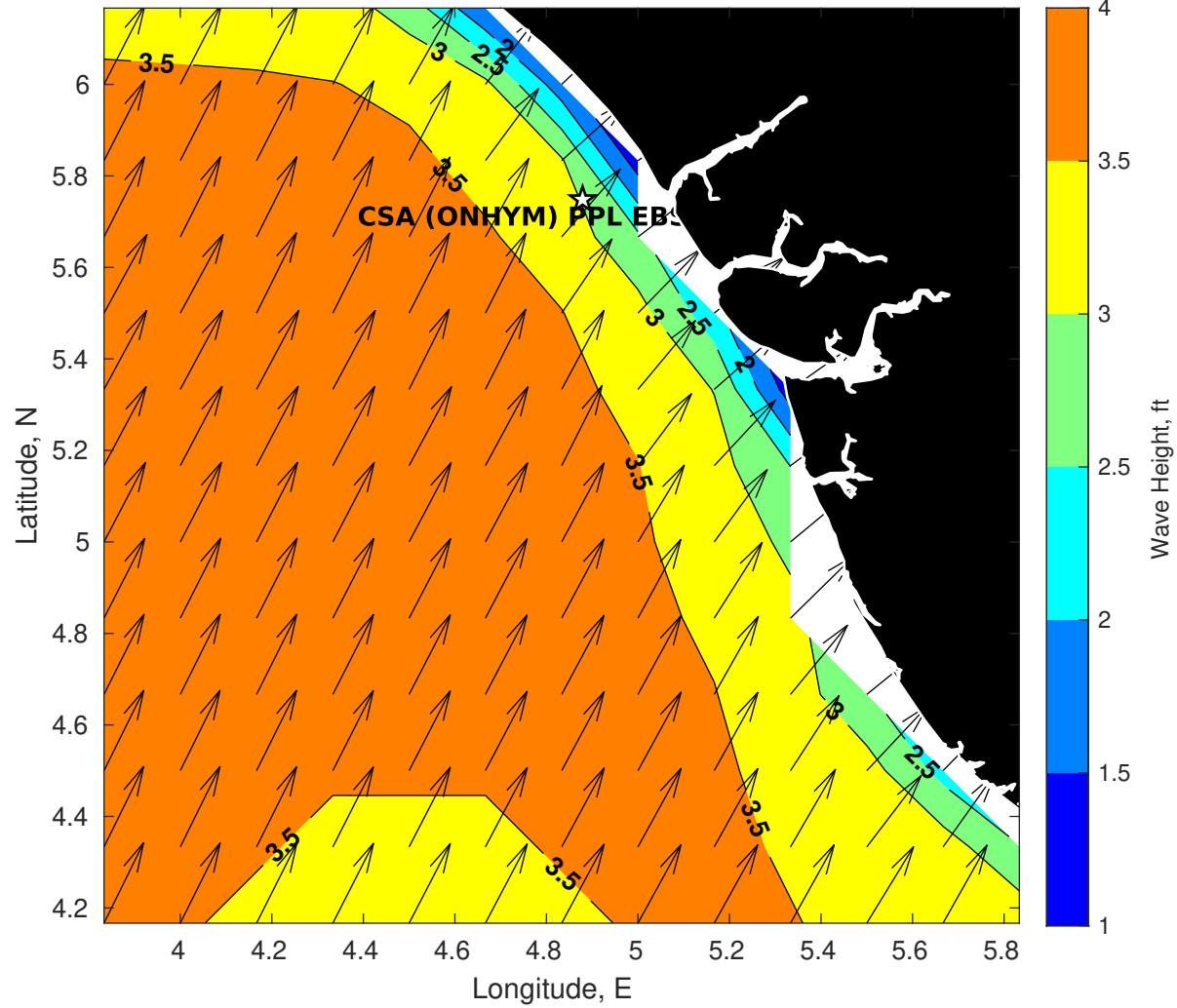
Wave Height (ft) for CSA (ONHYM) PPL EBS - Nigeria at 14-Sep-2025 09:00:00
