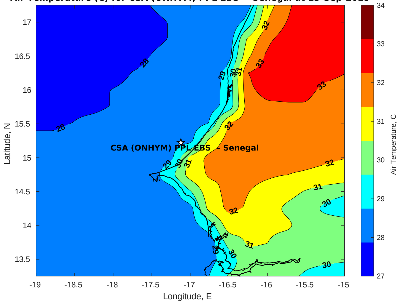
Air Temperature (C) for CSA (ONHYM) PPL EBS - Senegal at 13-Sep-2025
