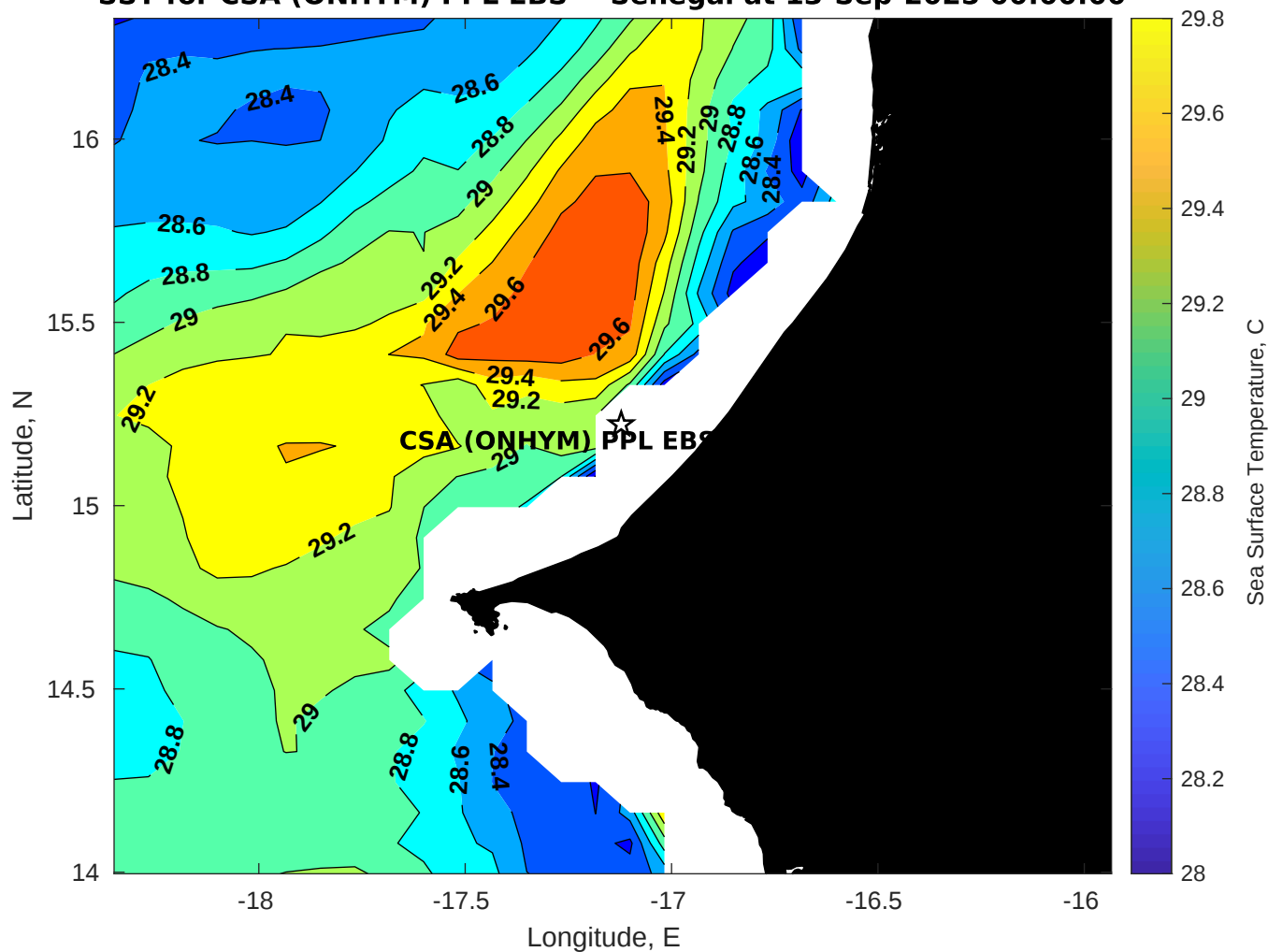
SST for CSA (ONHYM) PPL EBS - Senegal at 13-Sep-2025 00:00:00
