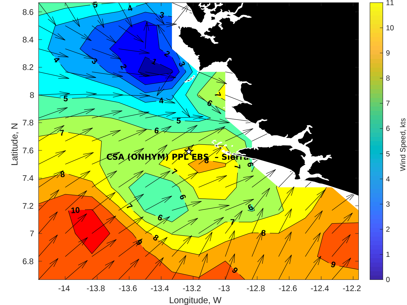
Winds (kts) for CSA (ONHYM) PPL EBS - Sierra Leone at 14-Sep-2025 09:00:00
