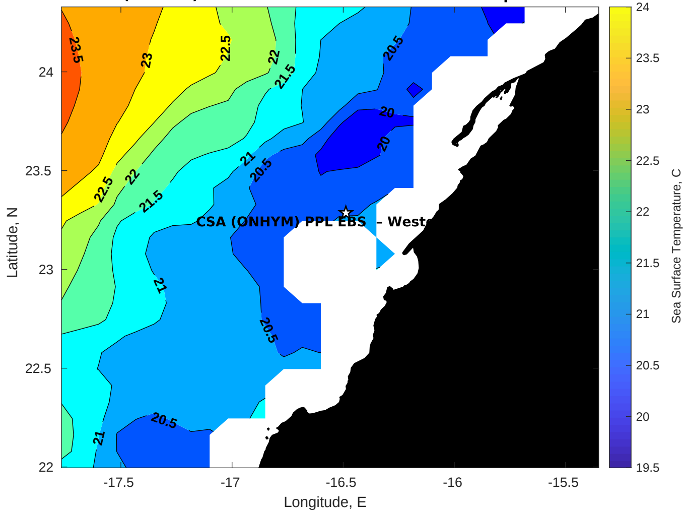
SST for CSA (ONHYM) PPL EBS - Western Sahara at 13-Sep-2025 00:00:00
