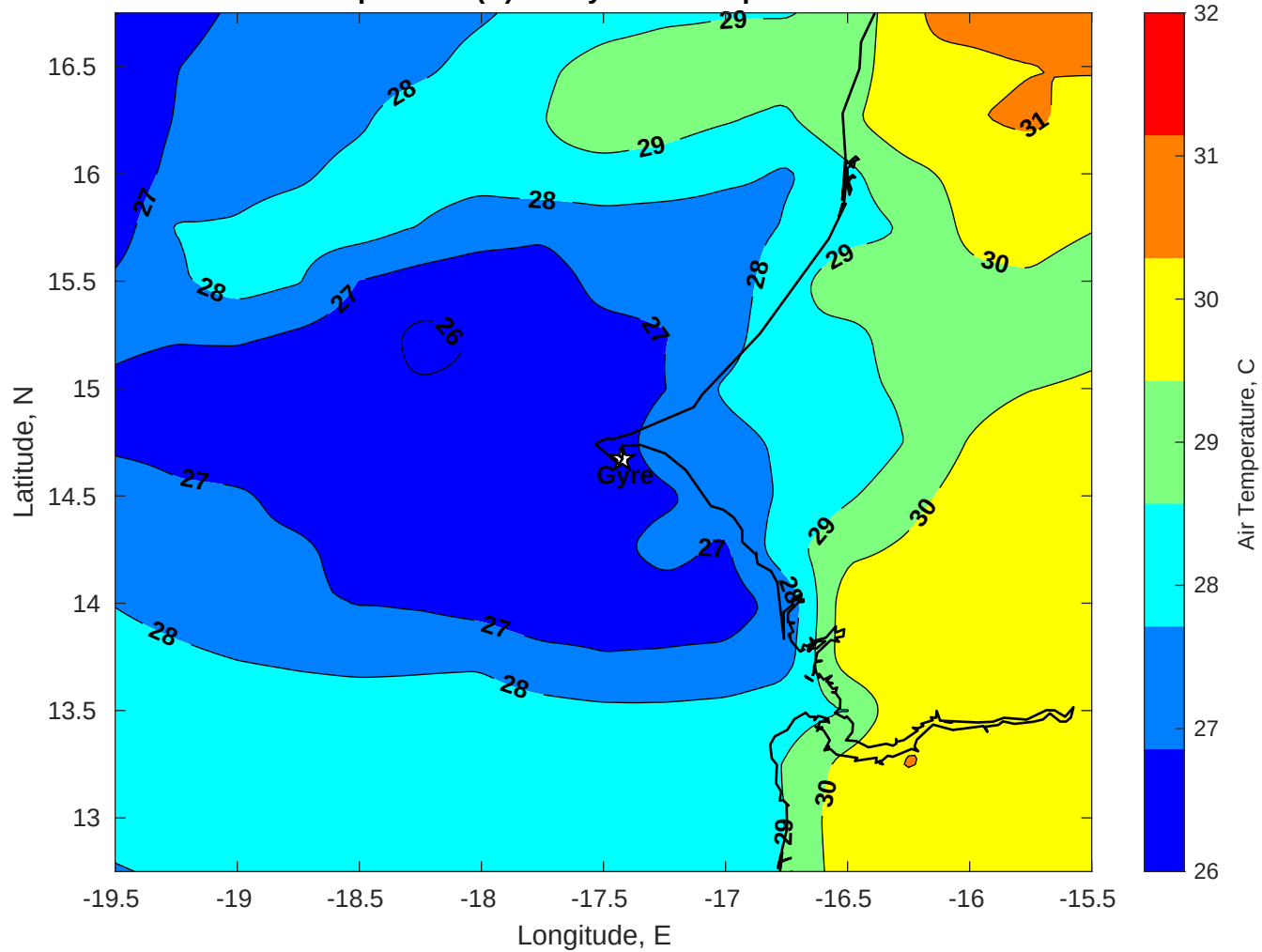
Air Temperature (C) for Gyre at 13-Sep-2025
