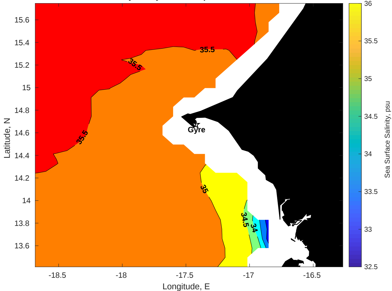
Surface Salinity for Gyre at 13-Sep-2025 00:00:00
