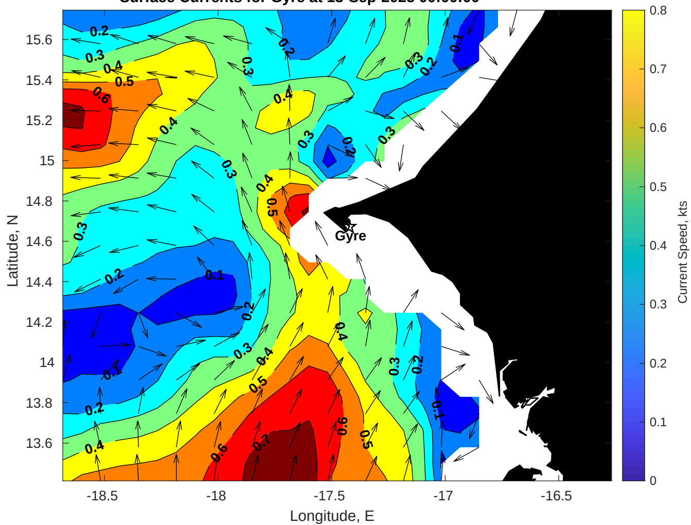
Surface Currents for Gyre at 13-Sep-2025 00:00:00
