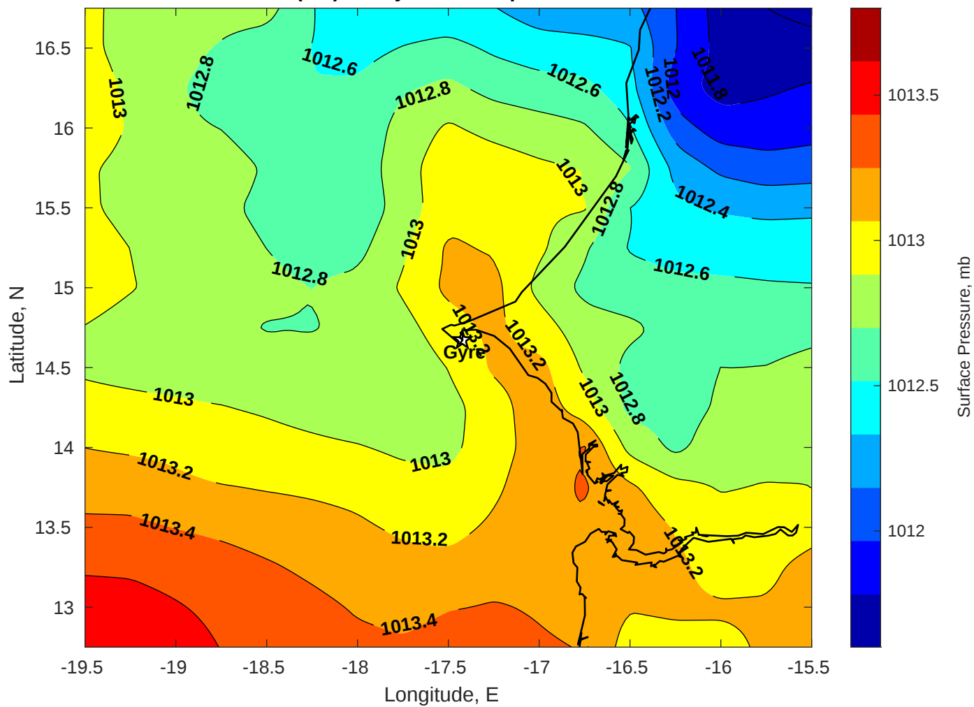
Surface Pressure (mb) for Gyre at 15-Sep-2025 12:00:00
