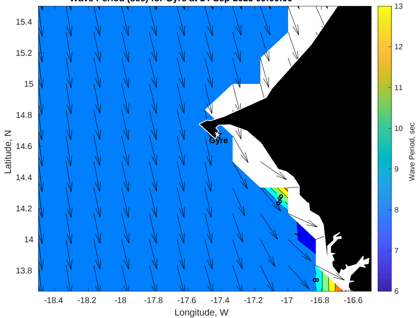
Wave Period (sec) for Gyre at 14-Sep-2025 09:00:00
