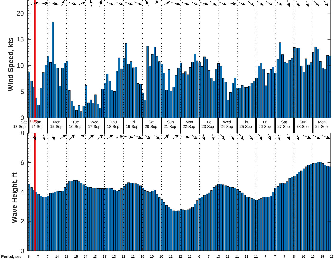
Wind & Wave Forecast for Gyre from 13-Sep-2025 23:00:00 to 29-Sep-2025 23:00:00
