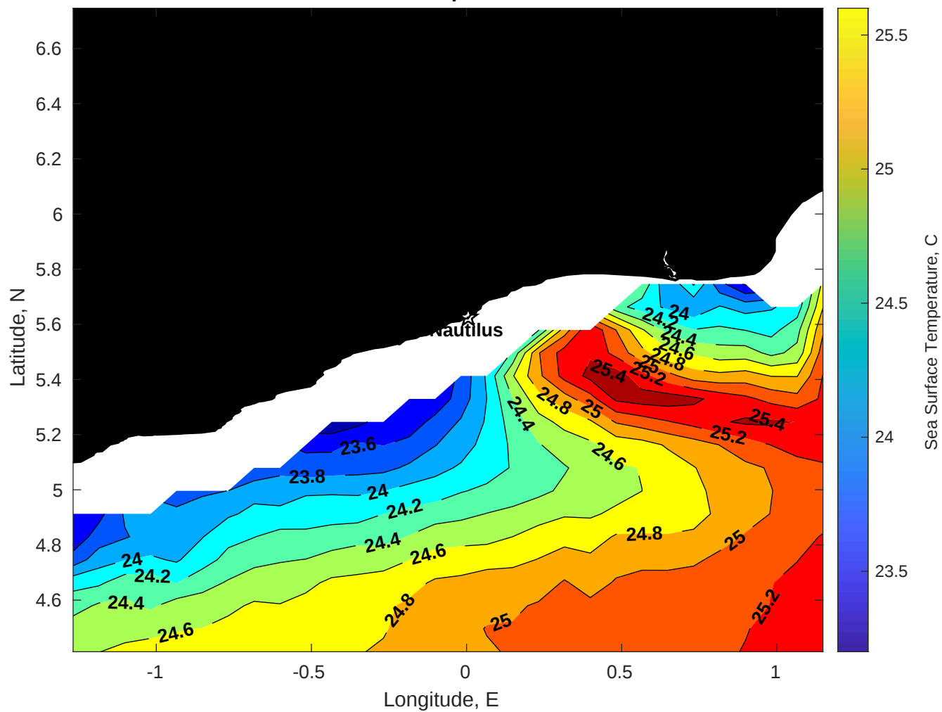
SST for Nautilus at 13-Sep-2025 00:00:00
