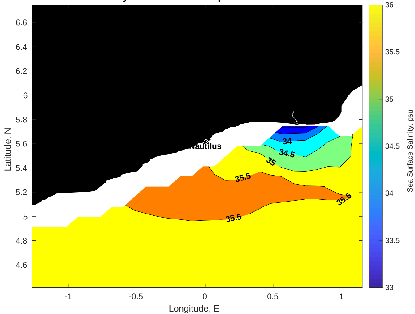
Surface Salinity for Nautilus at 13-Sep-2025 00:00:00
