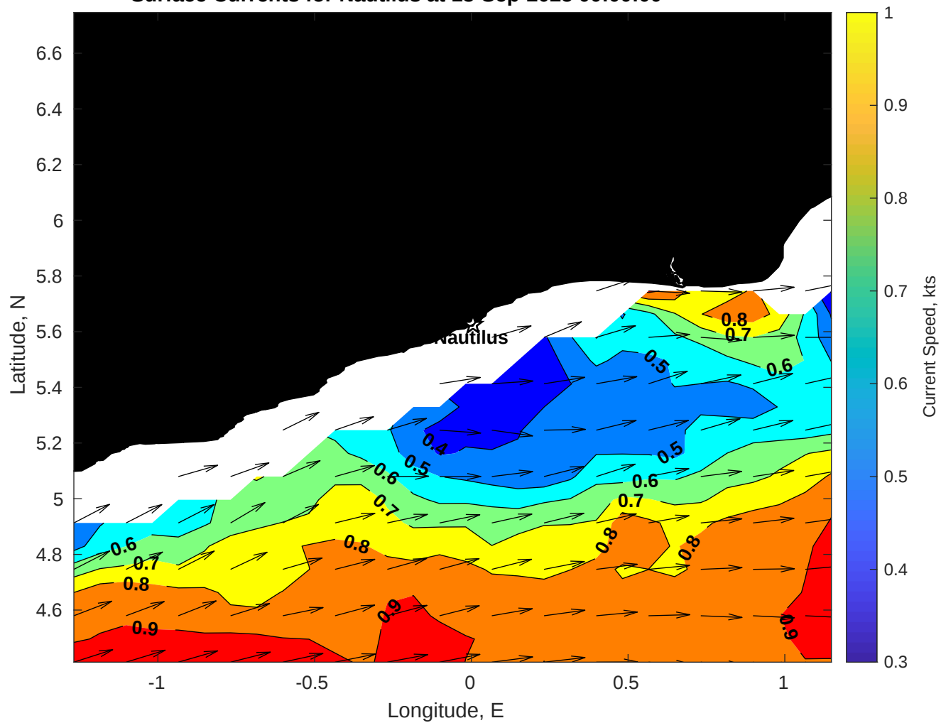
Surface Currents for Nautilus at 13-Sep-2025 00:00:00
