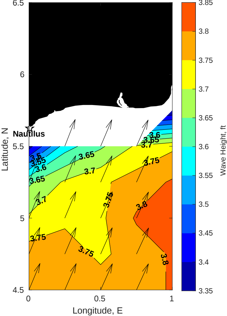
Wave Height (ft) for Nautilus at 14-Sep-2025 09:00:00
