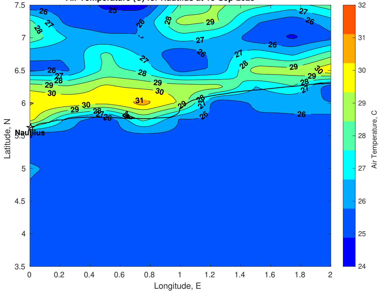
Air Temperature (C) for Nautilus at 13-Sep-2025
