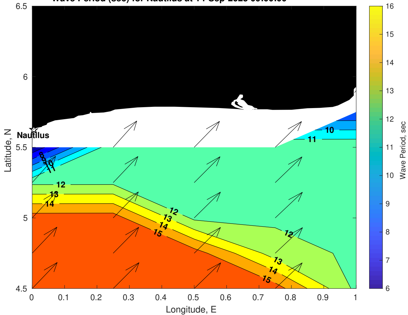
Wave Period (sec) for Nautilus at 14-Sep-2025 09:00:00
