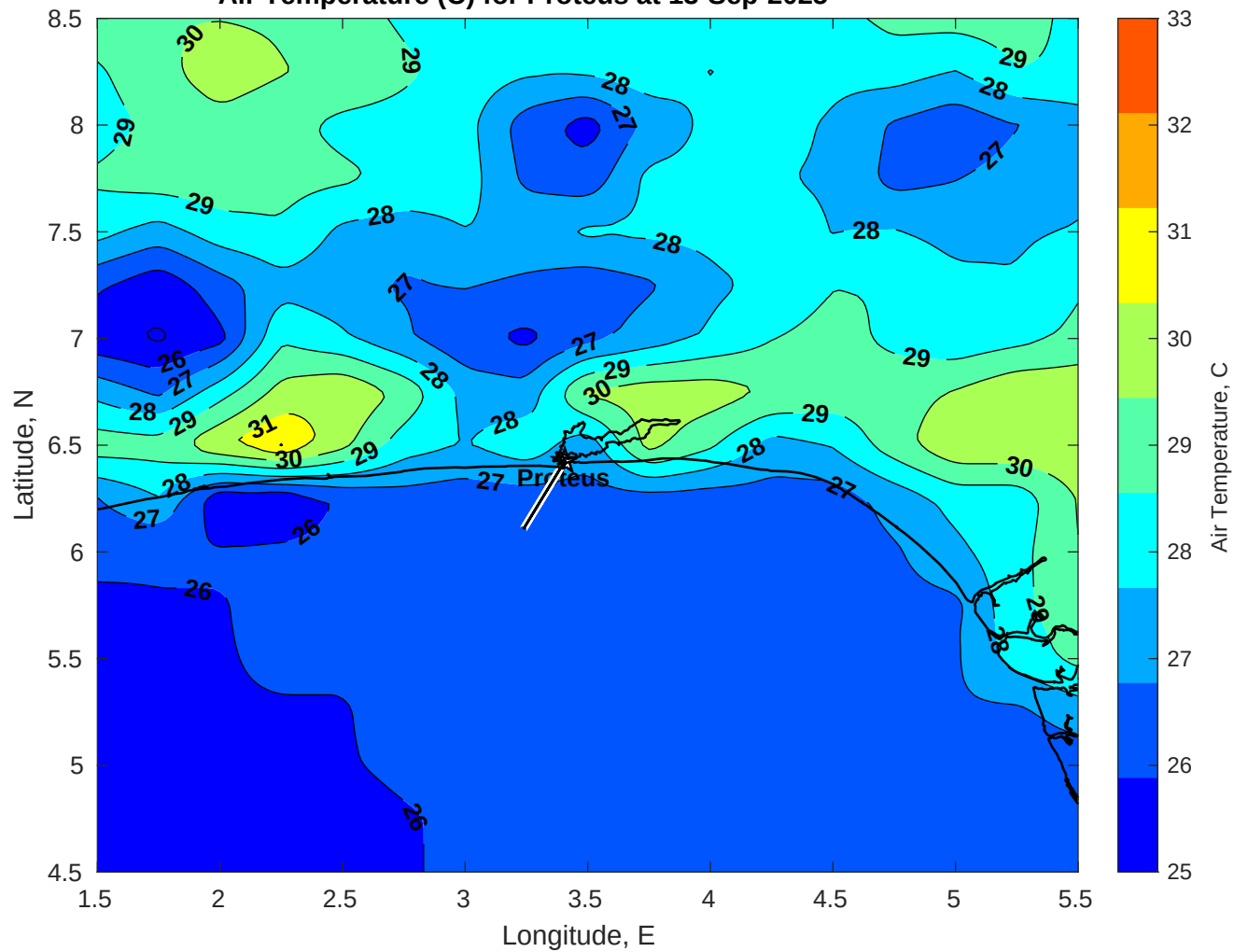
Air Temperature (C) for Proteus at 13-Sep-2025
