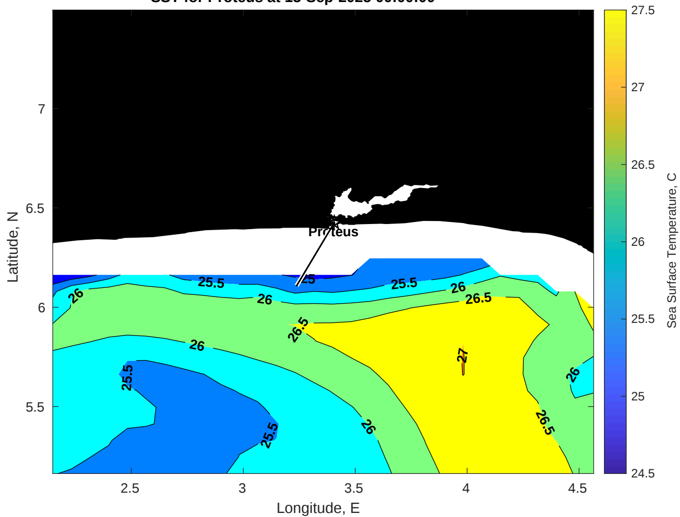
SST for Proteus at 13-Sep-2025 00:00:00
