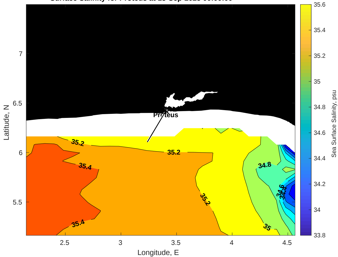
Surface Salinity for Proteus at 13-Sep-2025 00:00:00
