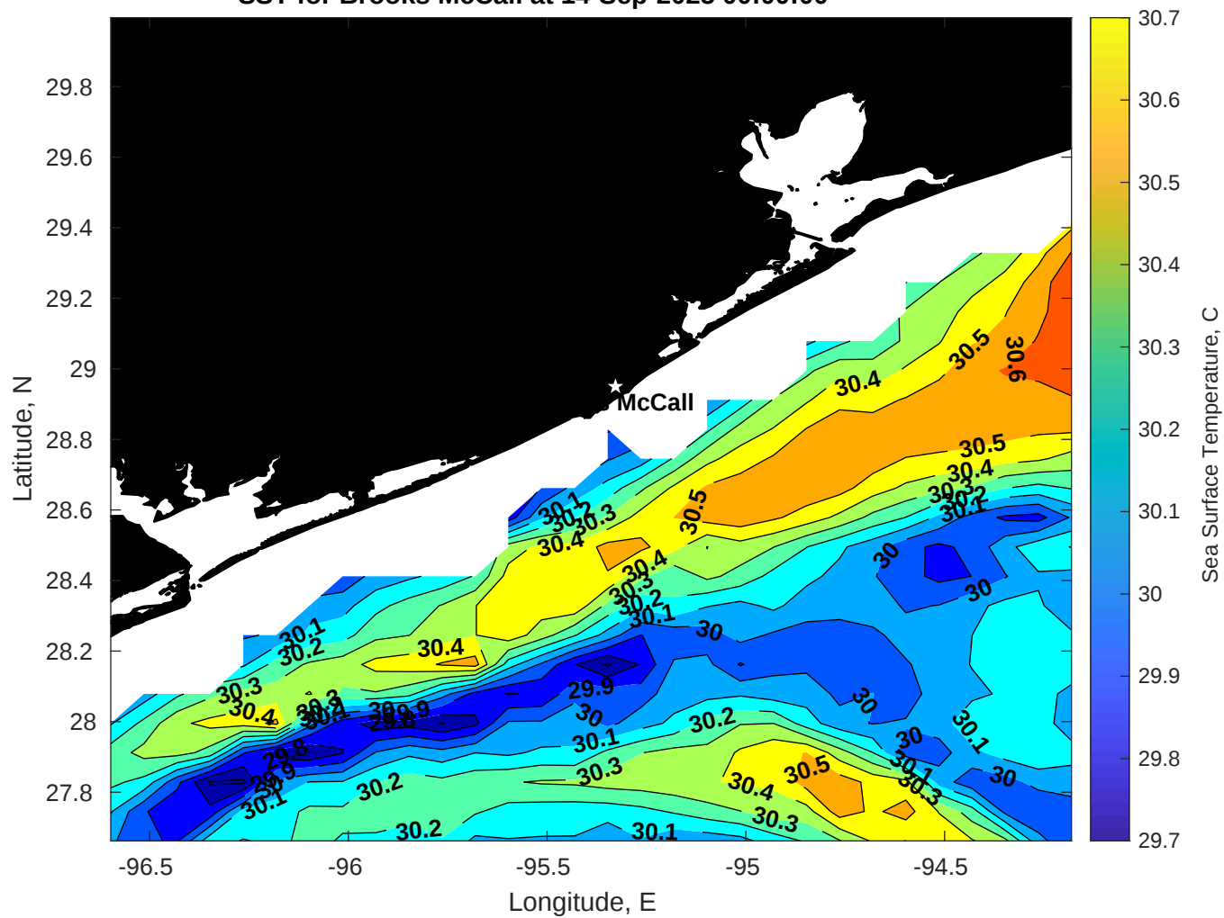
SST for Brooks McCall at 14-Sep-2025 00:00:00
