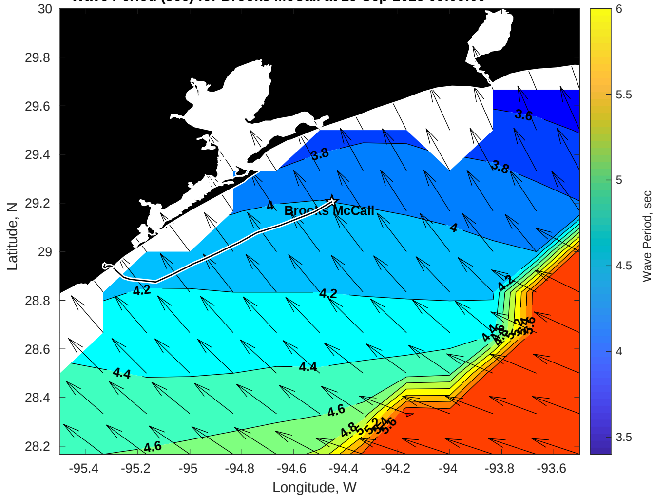
Wave Period (sec) for Brooks McCall at 15-Sep-2025 09:00:00
