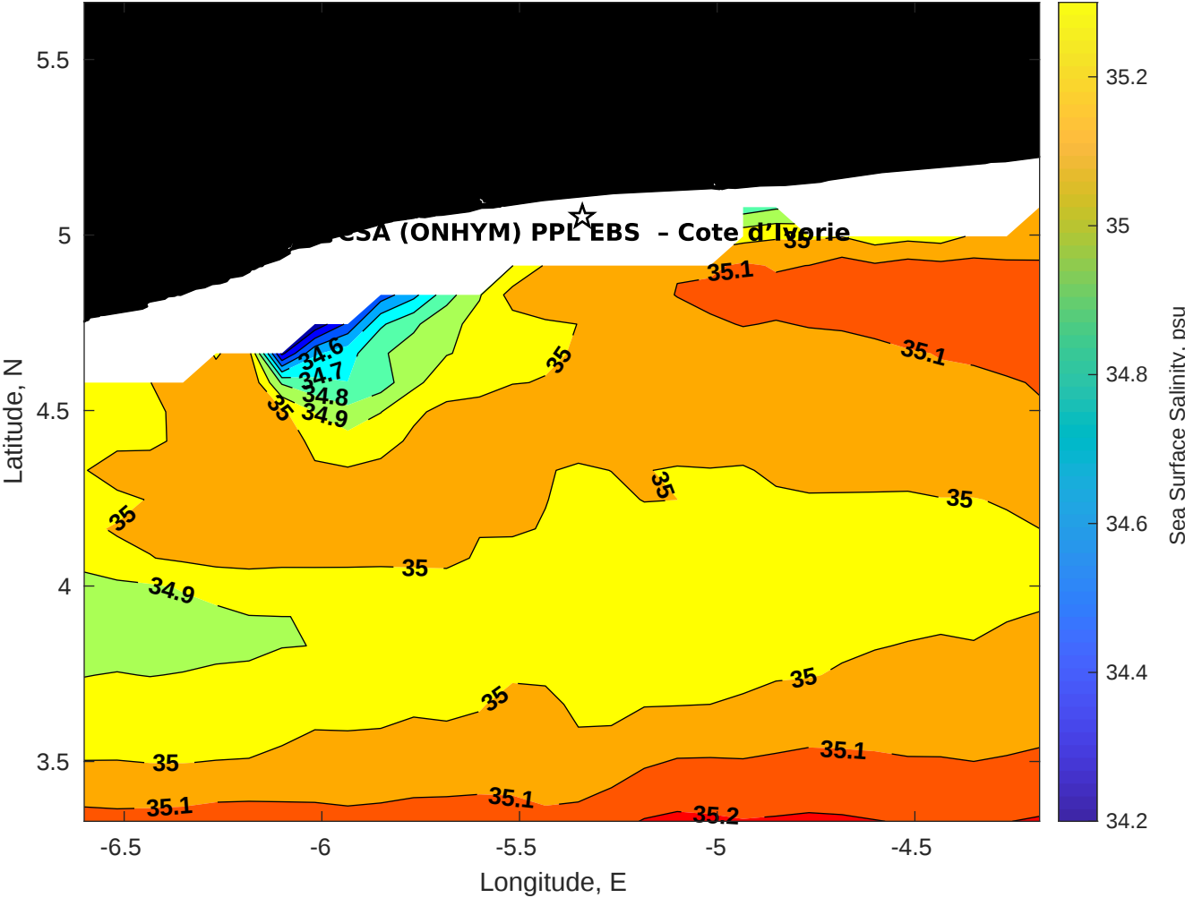
Surface Salinity for CSA (ONHYM) PPL EBS - Cote d'Ivoire at 14-Sep-2025 00:00:00
