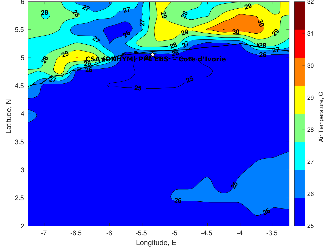
Air Temperature (C) for CSA (ONHYM) PPL EBS - Cote d'Ivoire at 14-Sep-2025
