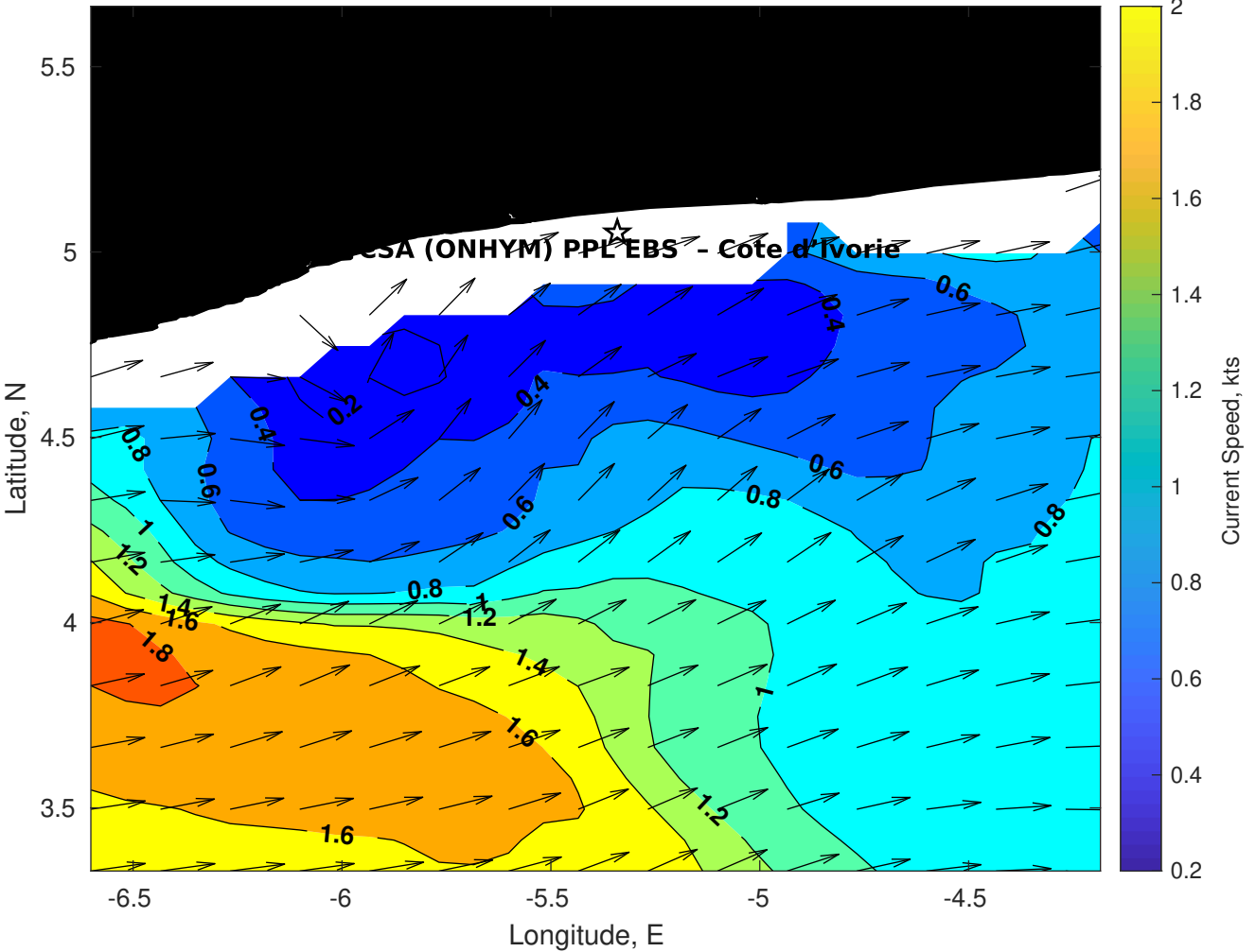
Surface Currents for CSA (ONHYM) PPL EBS - Cote d'Ivoire at 14-Sep-2025 00:00:00
