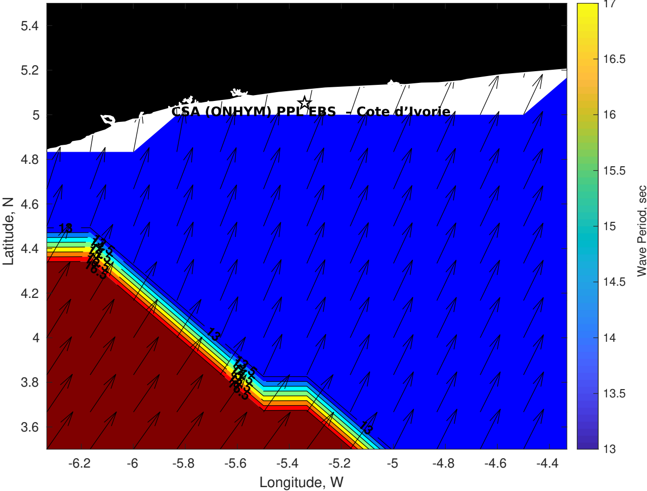
Wave Period (sec) for CSA (ONHYM) PPL EBS - Cote d'Ivoire at 15-Sep-2025 09:00:00
