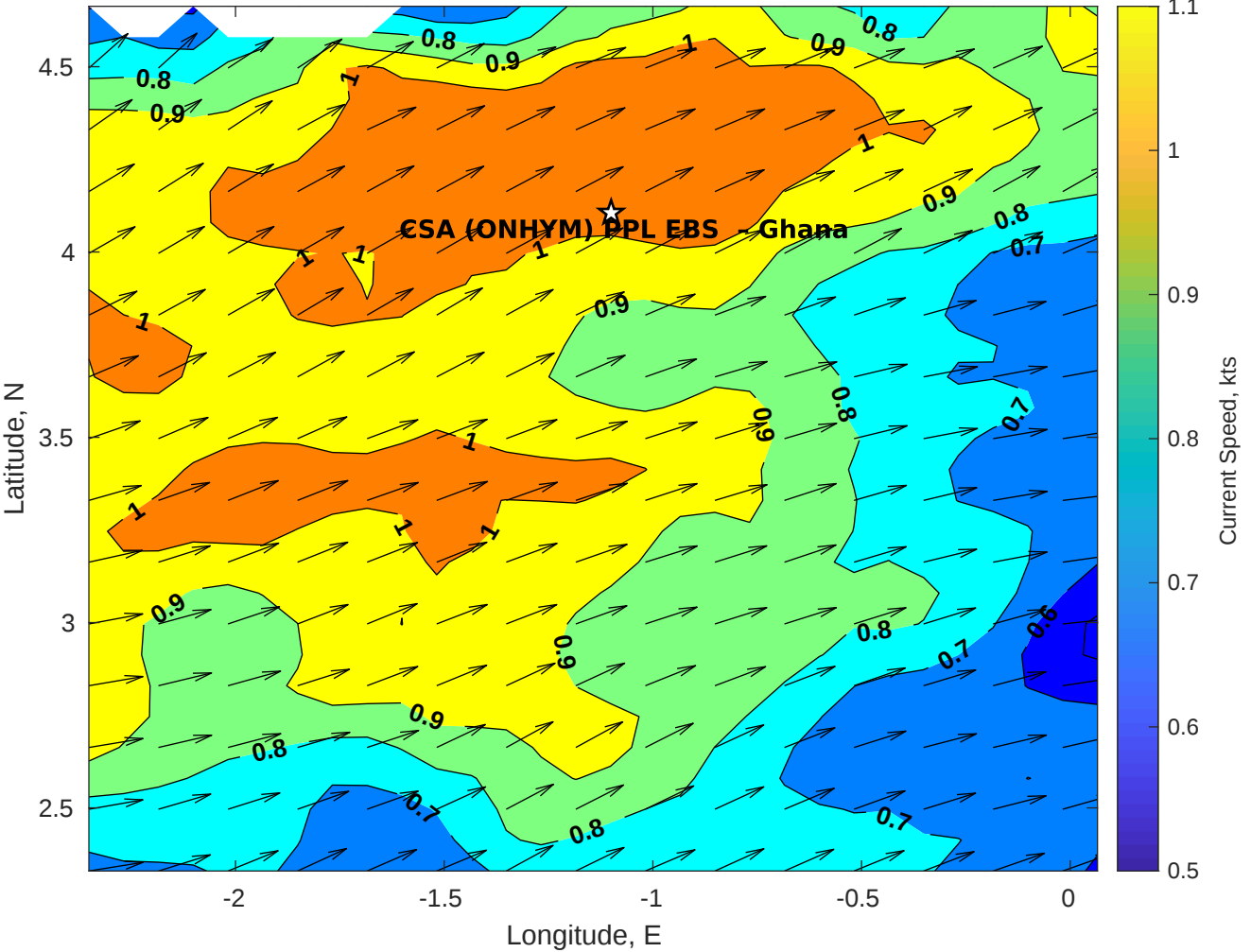
Surface Currents for CSA (ONHYM) PPL EBS - Ghana at 14-Sep-2025 00:00:00
