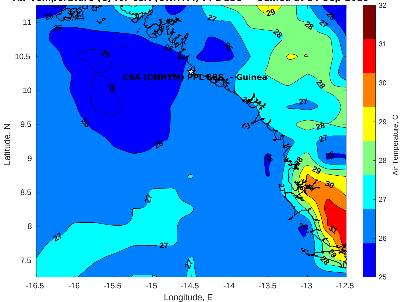
Air Temperature (C) for CSA (ONHYM) PPL EBS - Guinea at 14-Sep-2025
