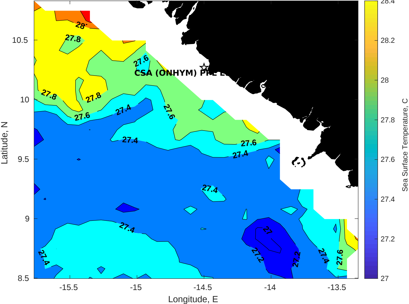
SST for CSA (ONHYM) PPL EBS - Guinea at 14-Sep-2025 00:00:00
