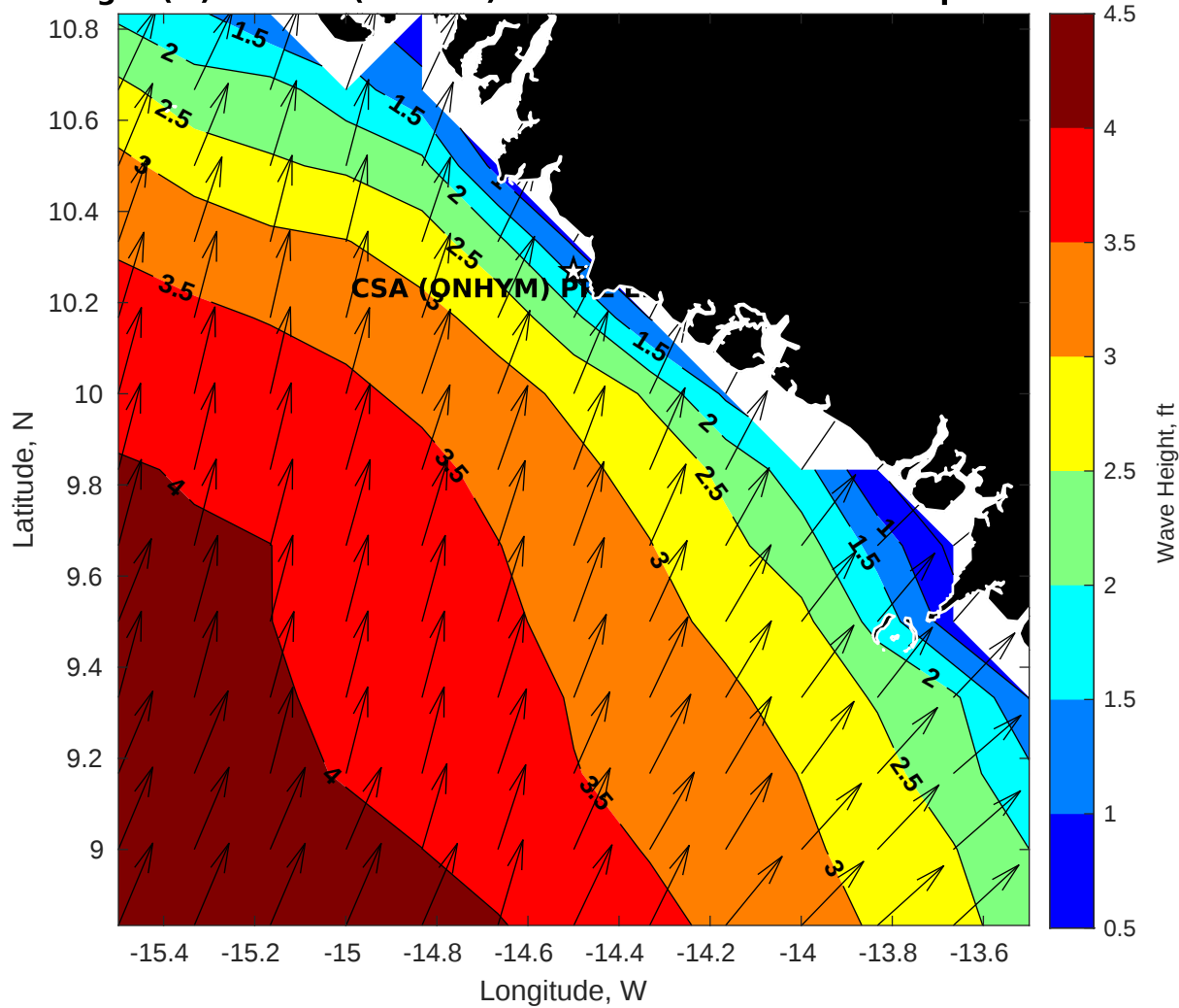
Wave Height (ft) for CSA (ONHYM) PPL EBS - Guinea at 15-Sep-2025 09:00:00
