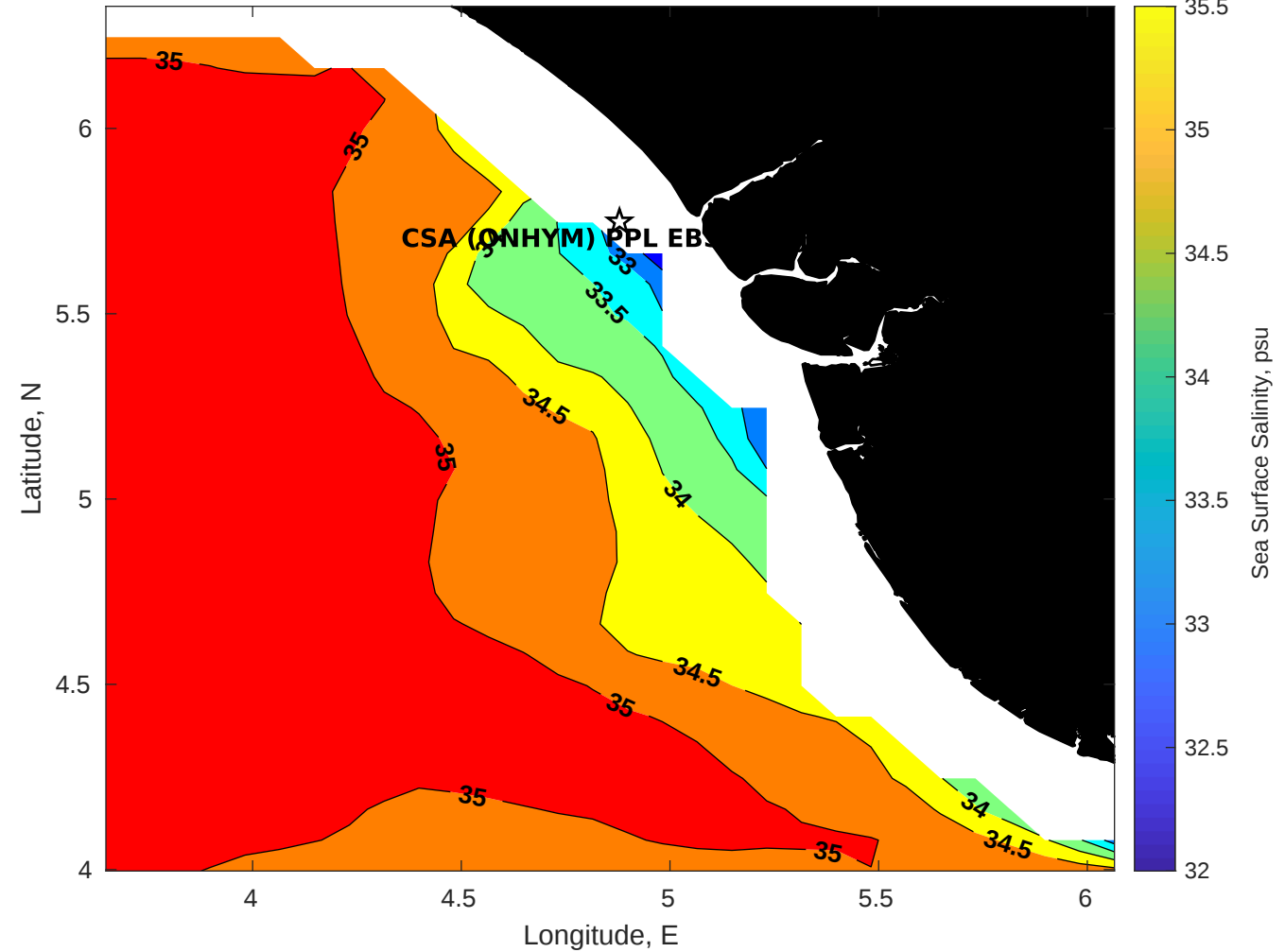
Surface Salinity for CSA (ONHYM) PPL EBS - Nigeria at 14-Sep-2025 00:00:00
