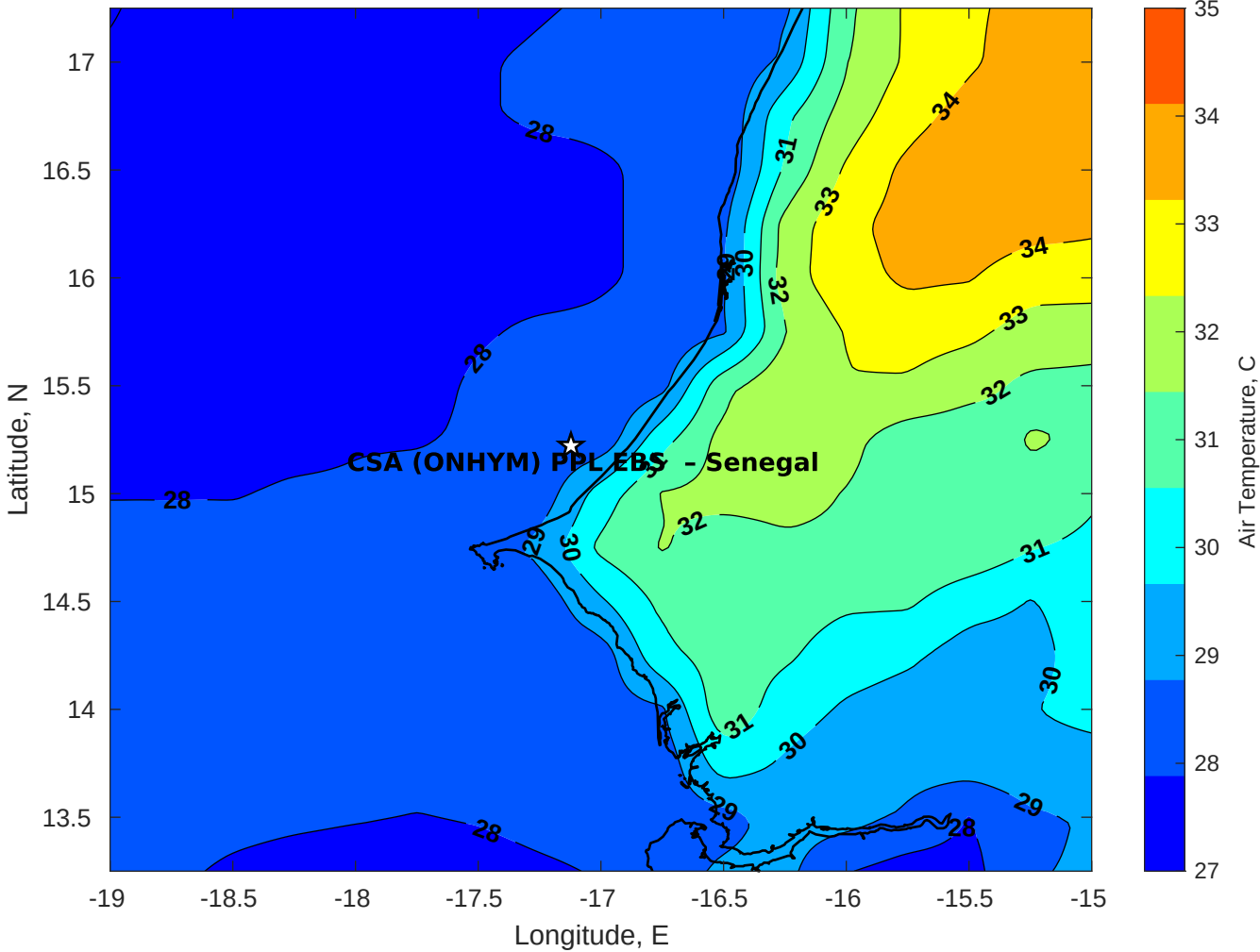
Air Temperature (C) for CSA (ONHYM) PPL EBS - Senegal at 14-Sep-2025
