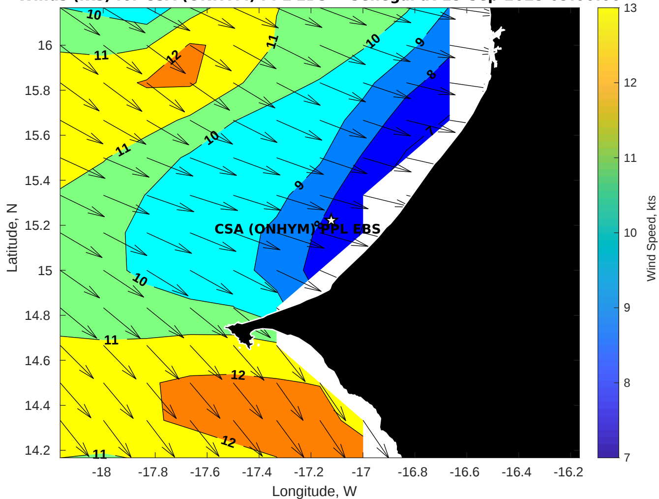
Winds (kts) for CSA (ONHYM) PPL EBS - Senegal at 15-Sep-2025 09:00:00
