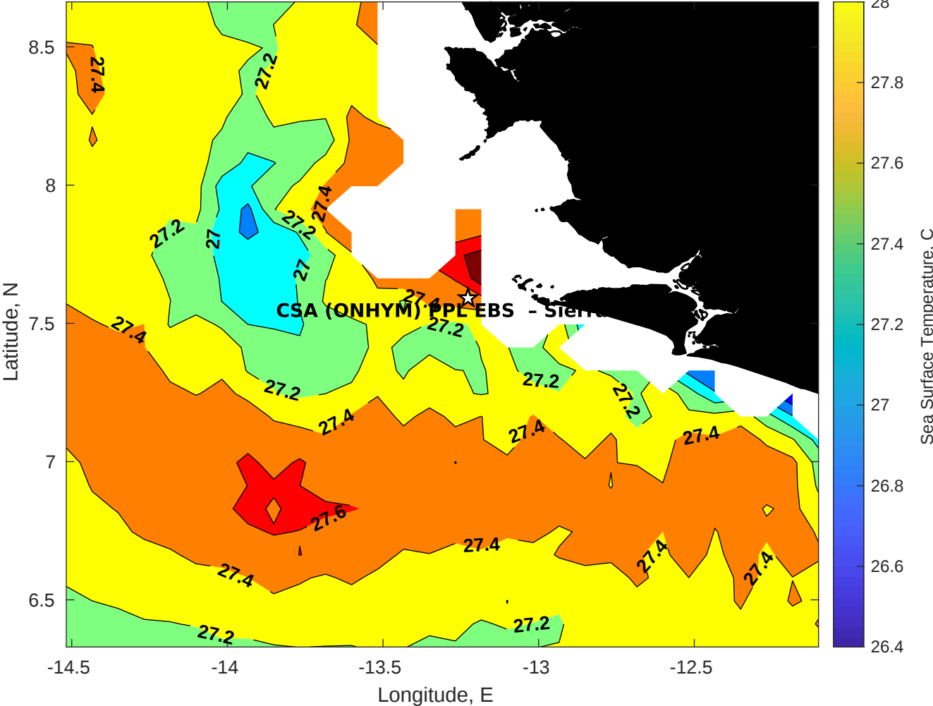
SST for CSA (ONHYM) PPL EBS - Sierra Leone at 14-Sep-2025 00:00:00
