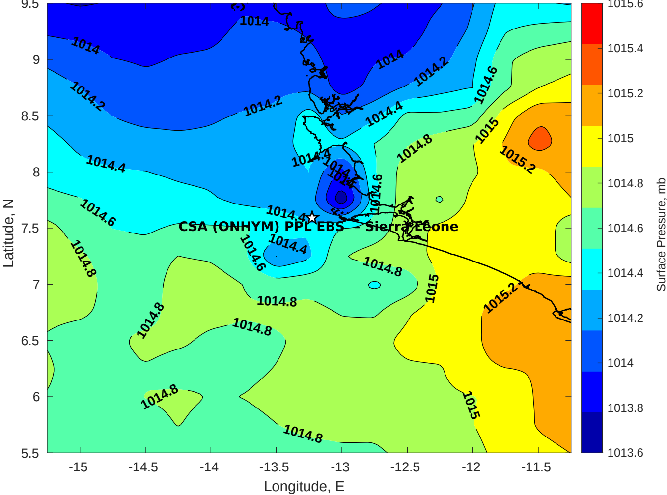
Surface Pressure (mb) for CSA (ONHYM) PPL EBS - Sierra Leone at 15-Sep-2025 12:00:00
