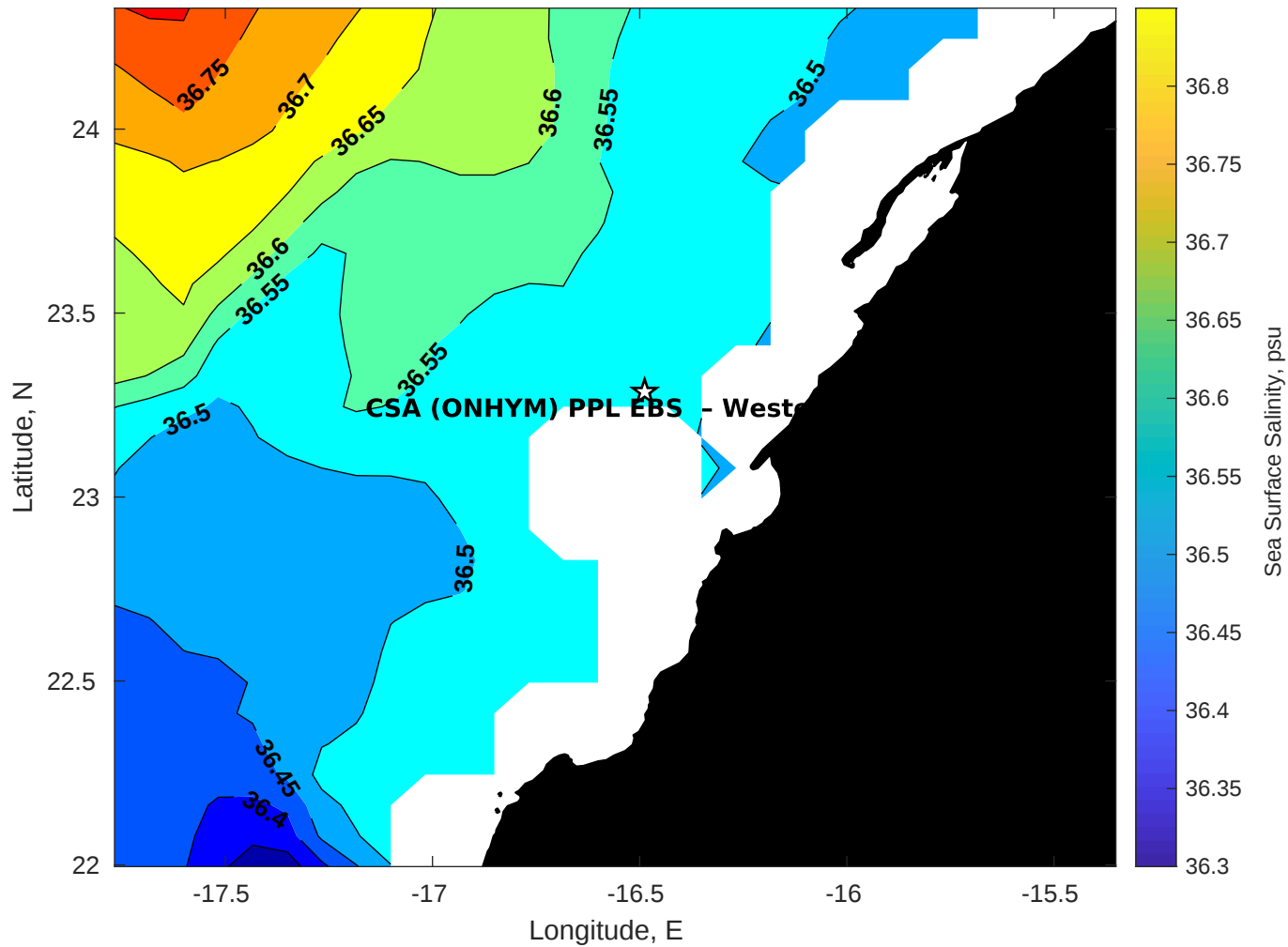
Surface Salinity for CSA (ONHYM) PPL EBS - Western Sahara at 14-Sep-2025 00:00:00
