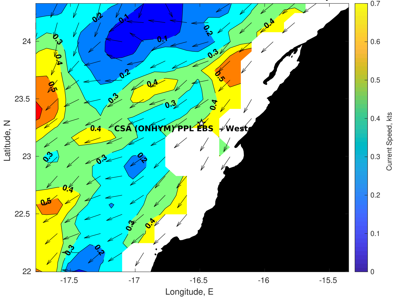
Surface Currents for CSA (ONHYM) PPL EBS - Western Sahara at 14-Sep-2025 00:00:00
