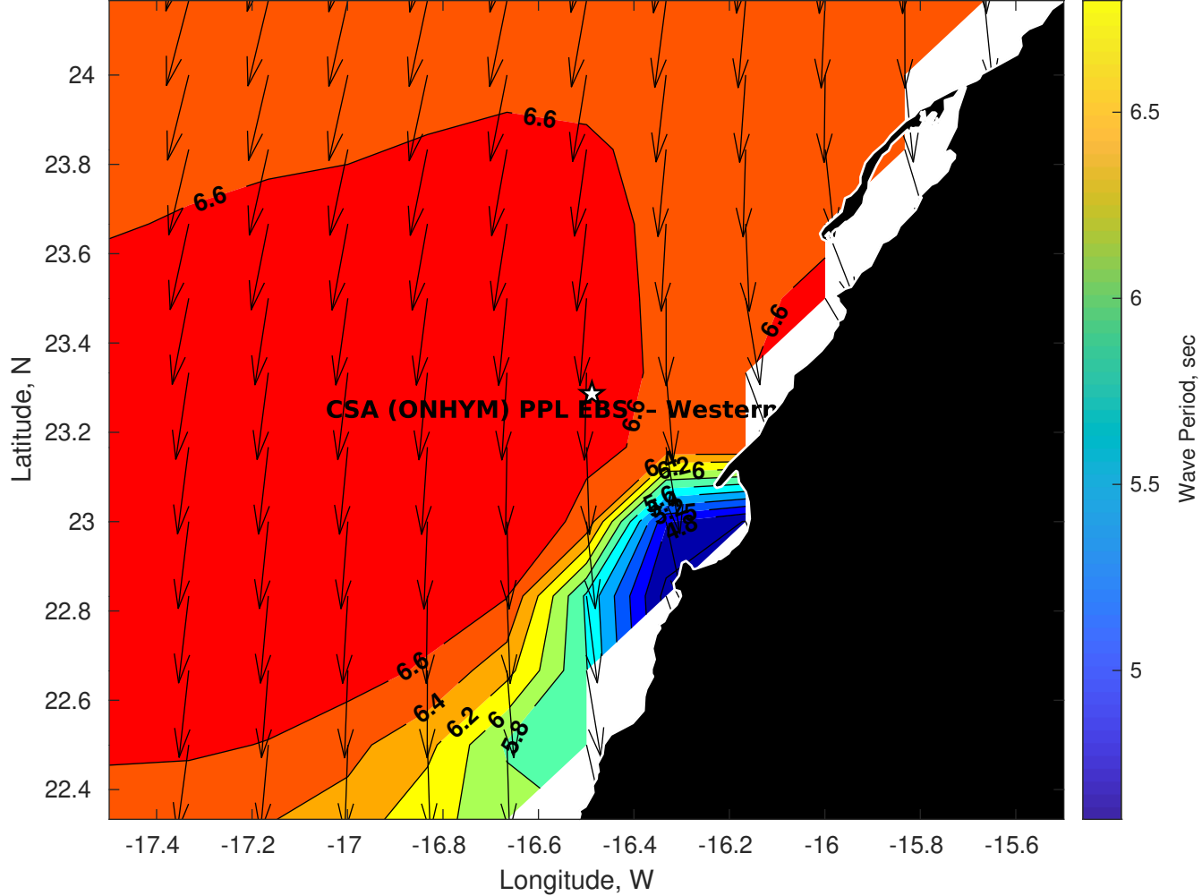
Wave Period (sec) for CSA (ONHYM) PPL EBS - Western Sahara at 15-Sep-2025 09:00:00
