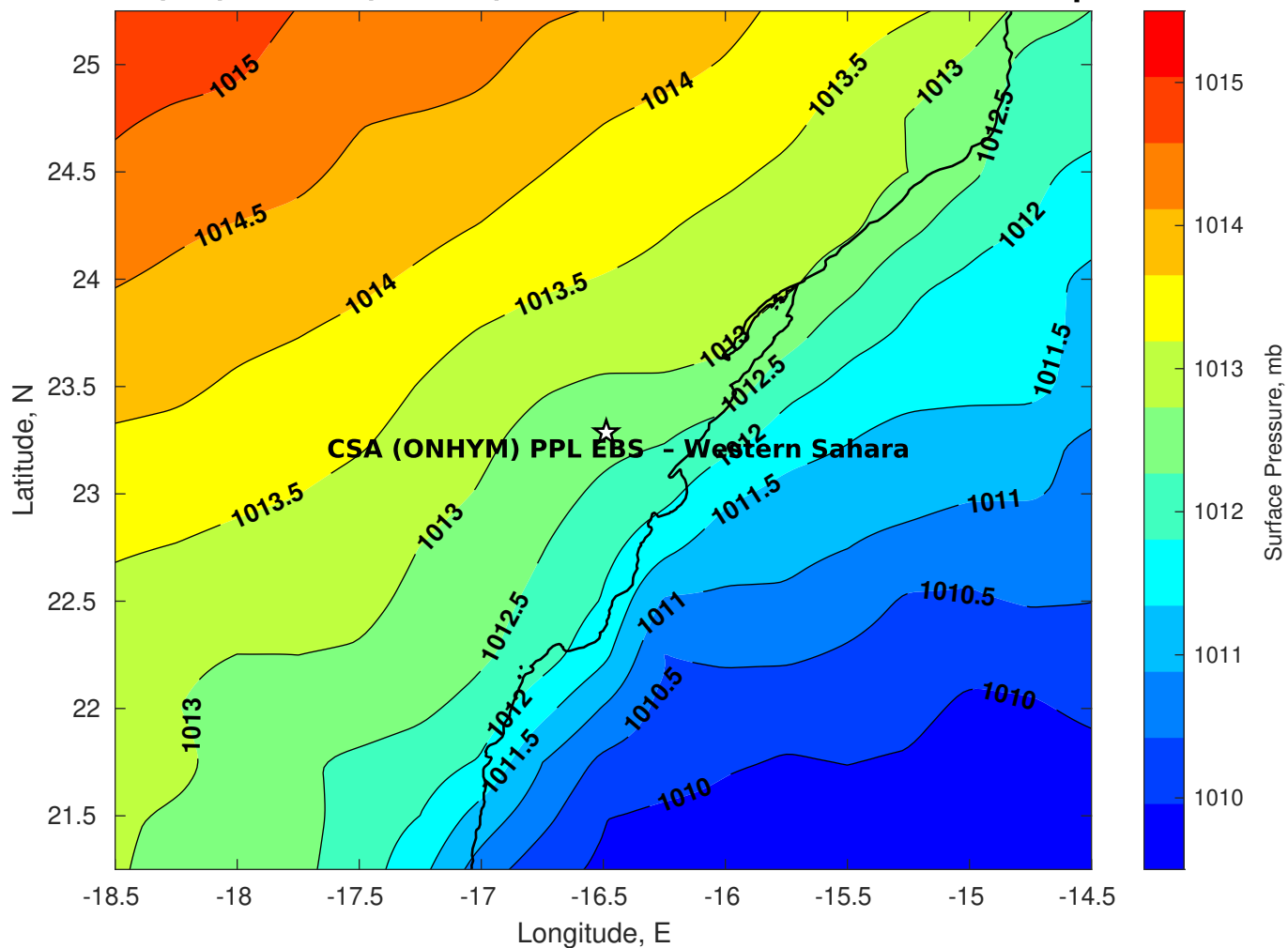
Surface Pressure (mb) for CSA (ONHYM) PPL EBS - Western Sahara at 15-Sep-2025 12:00:00
