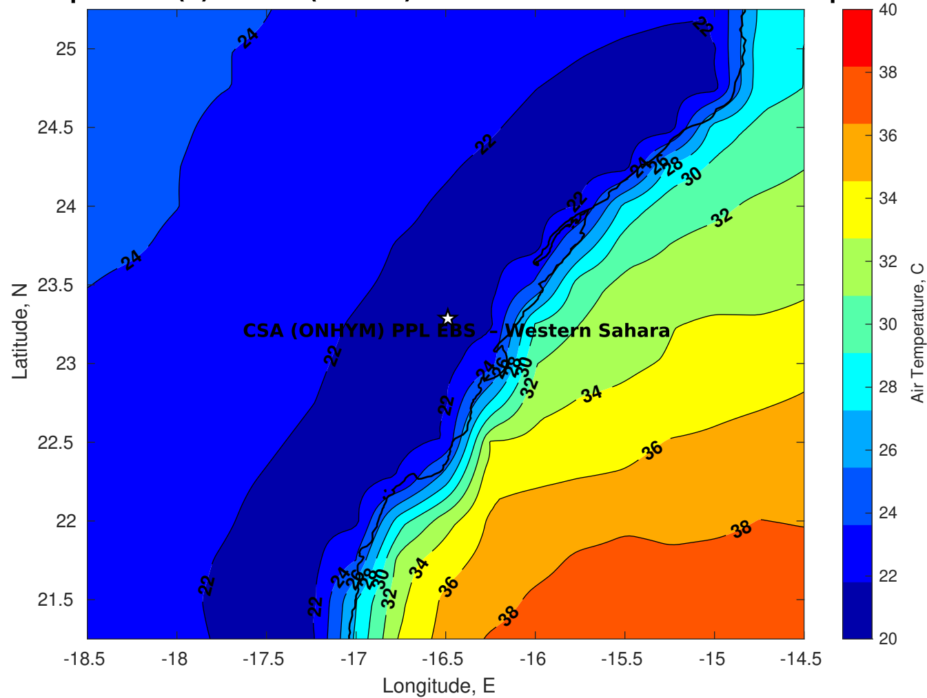
Air Temperature (C) for CSA (ONHYM) PPL EBS - Western Sahara at 13-Sep-2025
