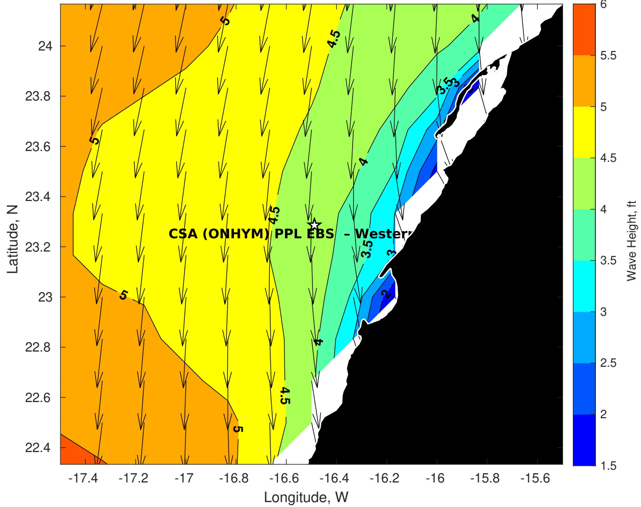
Wave Height (ft) for CSA (ONHYM) PPL EBS - Western Sahara at 15-Sep-2025 09:00:00
