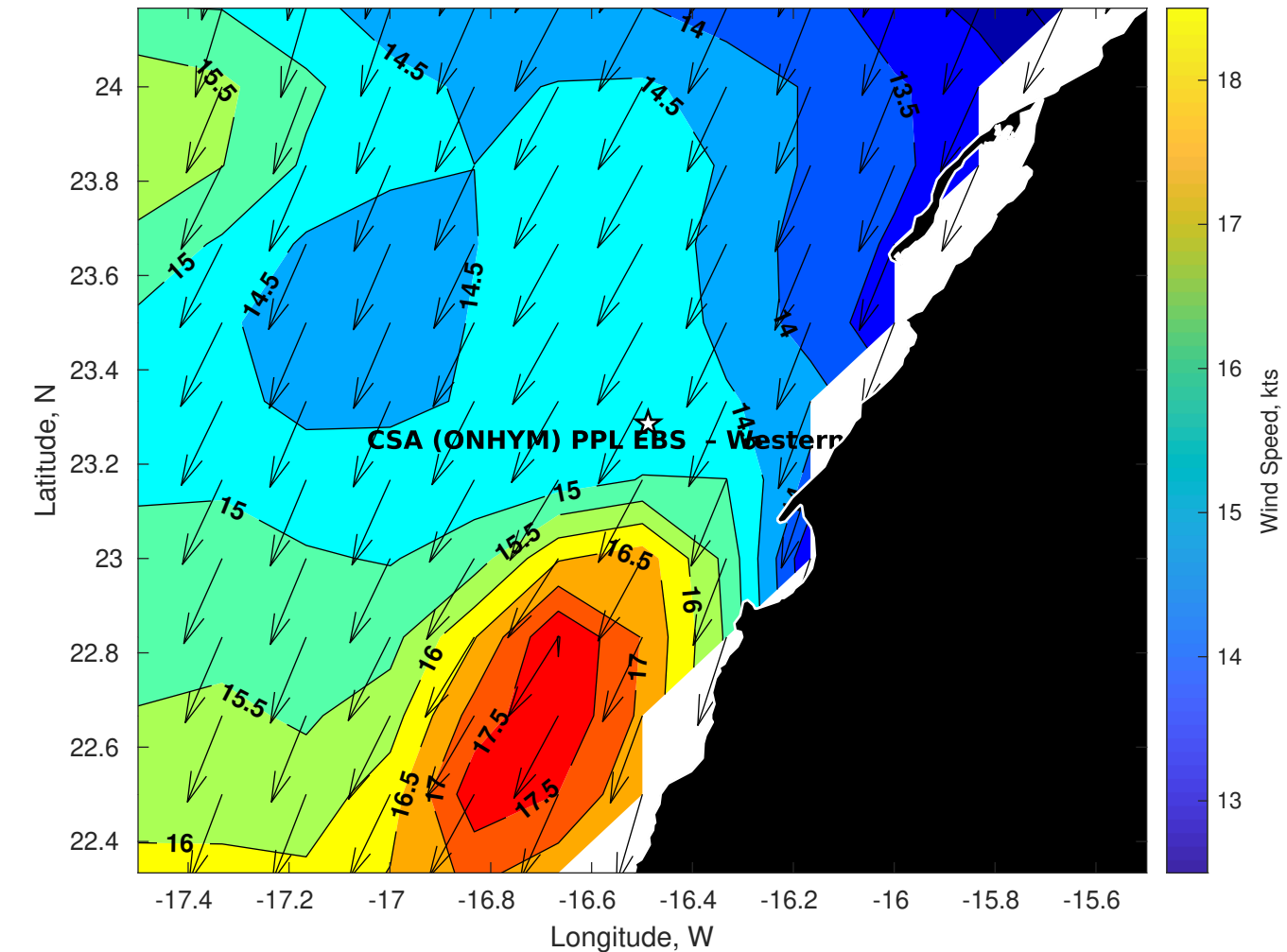
Winds (kts) for CSA (ONHYM) PPL EBS - Western Sahara at 15-Sep-2025 09:00:00
