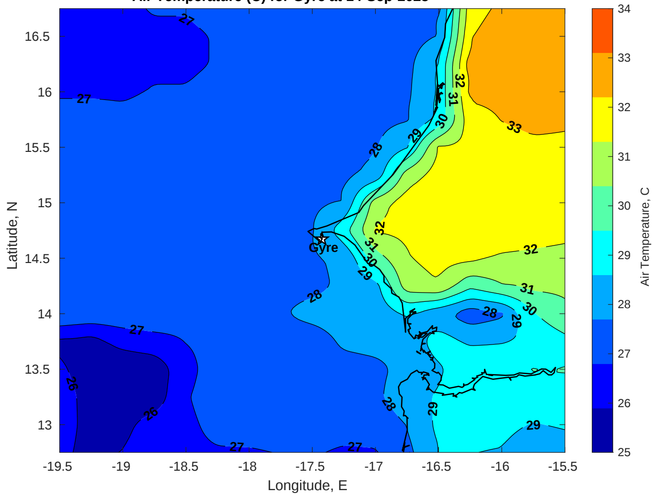
Air Temperature (C) for Gyre at 14-Sep-2025
