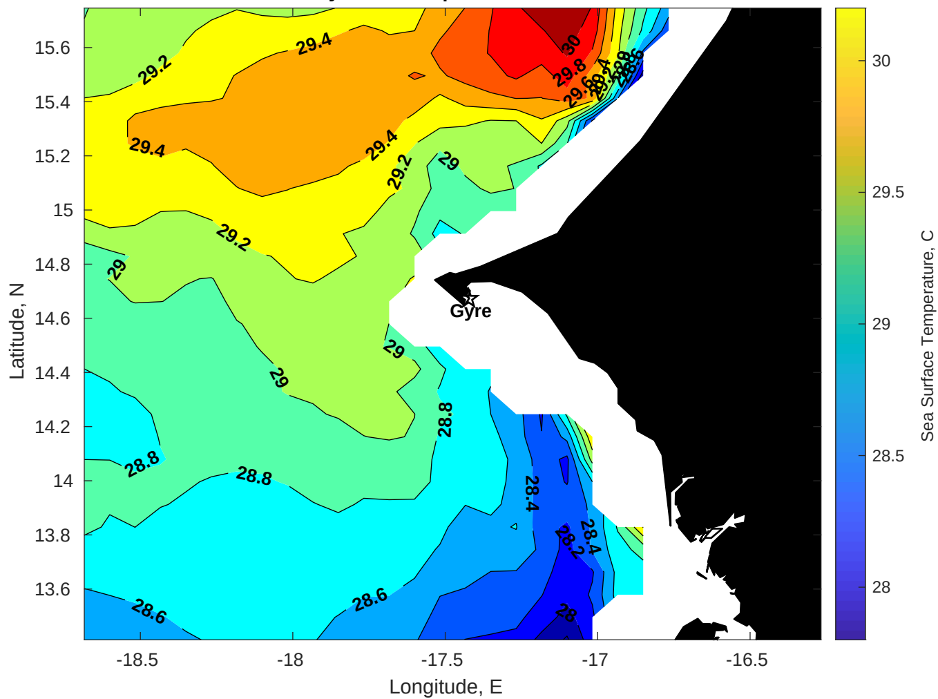
SST for Gyre at 14-Sep-2025 00:00:00
