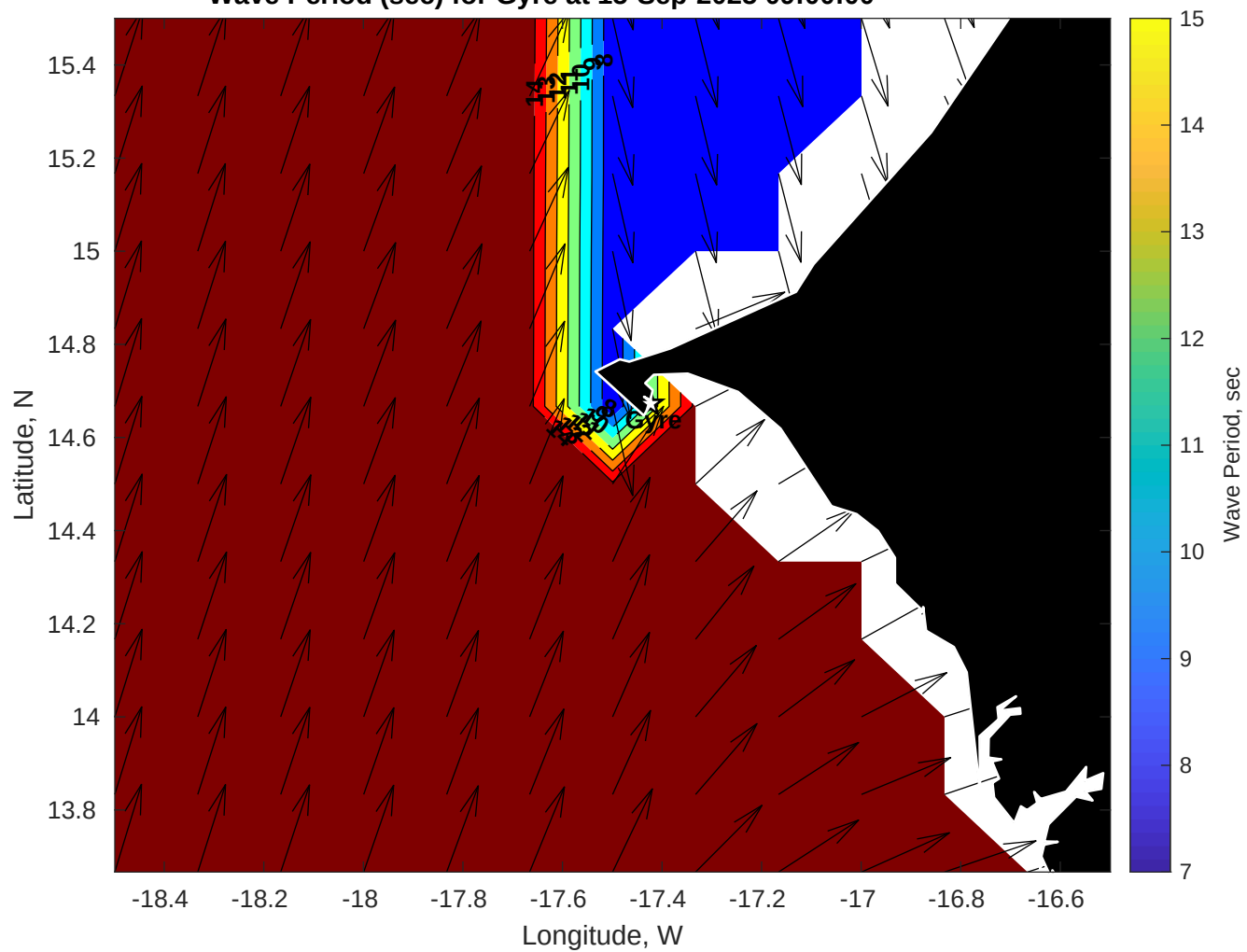
Wave Period (sec) for Gyre at 15-Sep-2025 09:00:00
