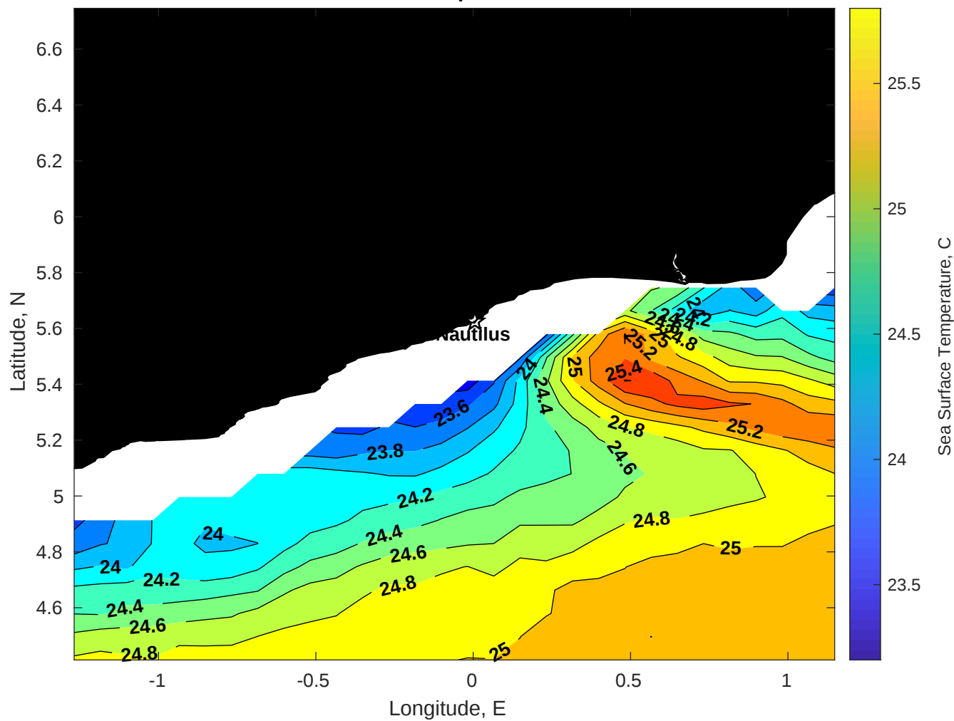
SST for Nautilus at 14-Sep-2025 00:00:00
