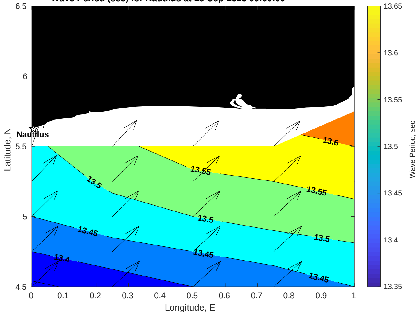
Wave Period (sec) for Nautilus at 15-Sep-2025 09:00:00
