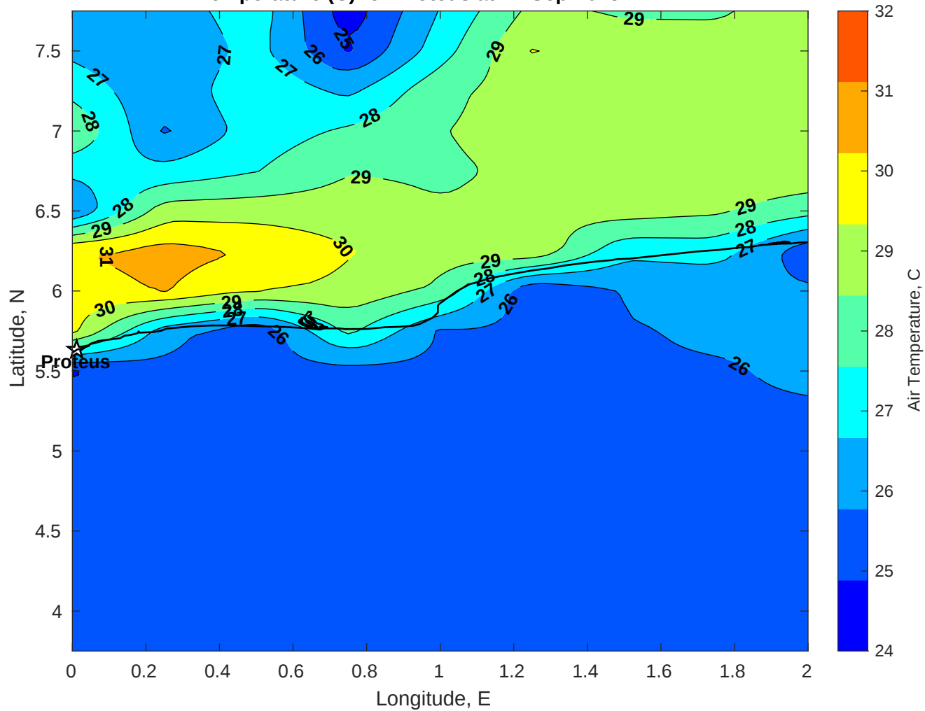
Air Temperature (C) for Proteus at 14-Sep-2025
